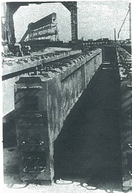
Fig. 26. Typical Tampa Bay beam in storage yard.
