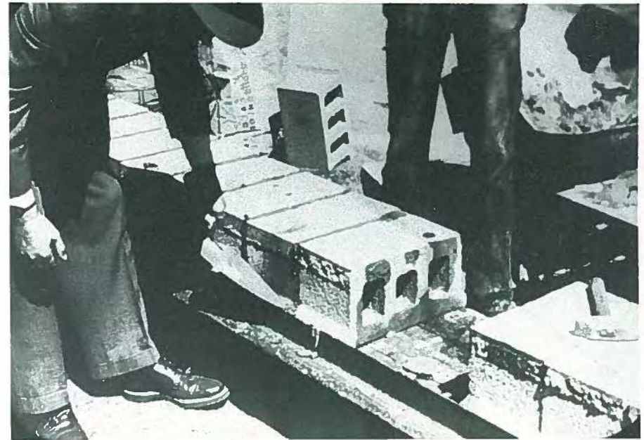
Fig. 7. Fabricating 8-in. (203 mm) block building beam.
