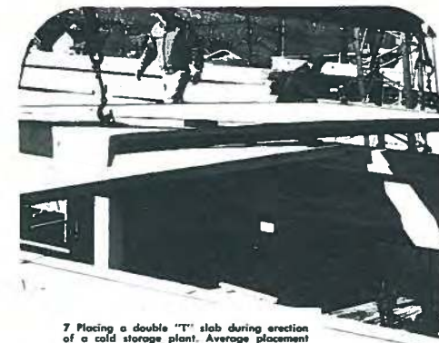
7 Placing a double "T" slab during erection of a cold storage plant. Average placement time was three minutes per slab.
