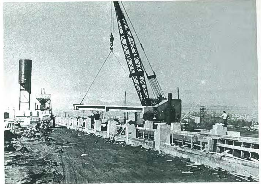
Fig. 11. A single-tee slab is lifted off the bed ready for transport to the Spitzer Electric Company.
