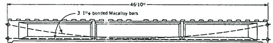
Fig. 25. Typical cross sections of prestressed concrete superstructure and elevation of prestressed beam for Tampa Bay Bridge (for contrast see Fig. 22). Note that this was the first use of the Lee-McCall system of prestressing in the United States.
