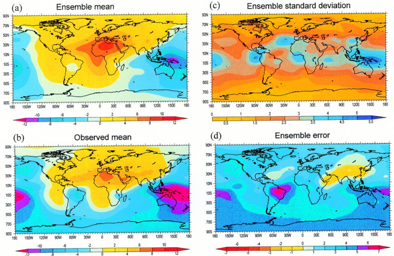
FIG. 2. As in Fig. 1 except for the velocity potential at 200 hPa ( 10^6 \text{ m}^2 \text{ s}^{-1} ).
