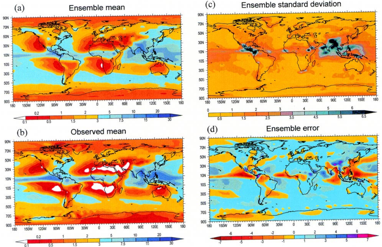
FIG. 4. As in Fig. 3 except for JJA.
