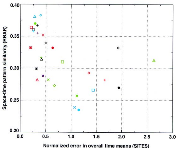
FIG. 15. A model performance diagram showing the AMIP models' simulation of the mean DJF sea level pressure during 1979–88 in terms of the normalized error of the time mean (SITES) and the evolution of the space–time pattern (RBAR), relative to the ECMWF reanalysis. (The DNM model's location at SITES = 9.35 and RBAR = 0.14 is not shown.)
