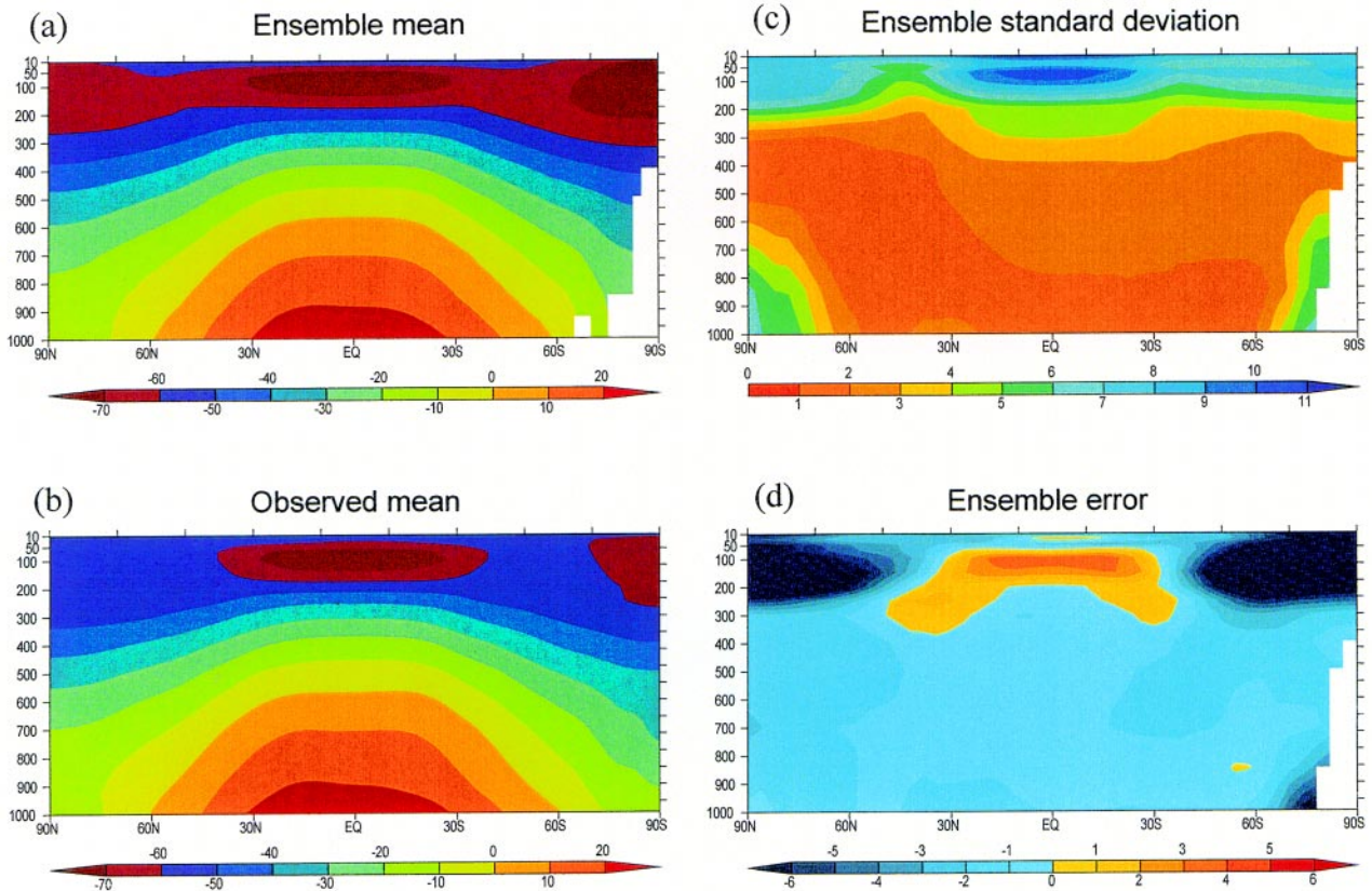
FIG. 8. (a) The latitude–pressure meridional section of the temperature ( ^{\circ}\text{C} ) given by the AMIP ensemble mean and (b) the observed data from the ECMWF reanalysis (Gibson et al. 1997). (c) The standard deviation of the ensemble mean. (d) The ensemble error. The pressure units are hPa.
