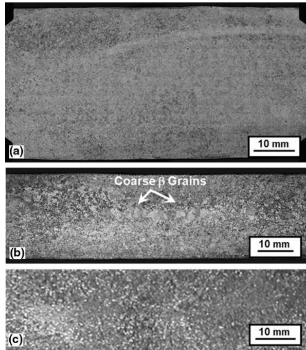
Fig. 27—Macrographs of transverse sections of sidepressed Ti64 cylindrical preforms which were \beta annealed at 1311 K ( 1038^\circ\text{C} ) for 1 hour following subtransus forging at (a, b) 1228 K ( 955^\circ\text{C} ) or (c) 1186 K ( 913^\circ\text{C} ) to a reduction of (a) \sim 40 pct. or (b, c) \sim 65 pct.
