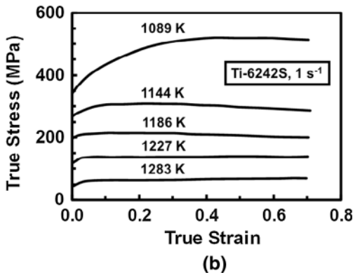
Fig. 3—Deformation-heating-corrected flow curves for (a) the single-phase \alpha alloys Ti-6.9Al and Ti-6.9Al-1.6V and (b) Ti6242 in the \alpha + \beta phase field ( T \leq 1227 \text{ K} (954 °C) or \beta field [ T = 1283 \text{ K} (1010 °C)]). [21] All alloys had an equiaxed- \alpha starting microstructure.
