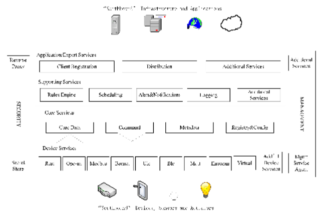
FIGURE 2. EdgeX foundry architecture.
