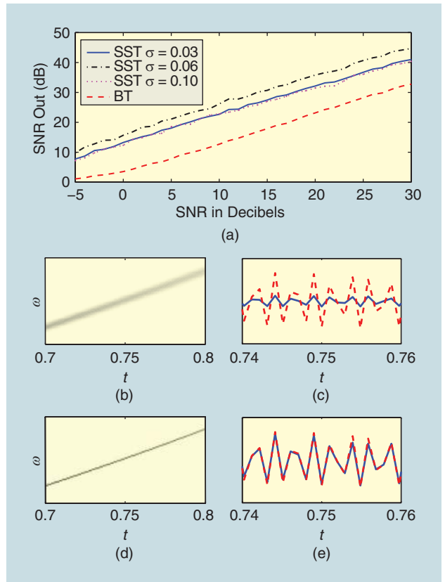
[FIG6] (a) Denoising results using the algorithm in the section “Denoising Multicomponent Signals Using SST” but using \tilde{T}_r^c (the parameter d being still fixed to 8 rad/s). (b) |T_r^c| of the signal in Figure 2(b). (c) Reconstructed mode from (b) (solid line) and the ground truth f_3 (dashed line), with d = 1 rad/s. (d) The same as (b) but using T_r^c instead of \tilde{T}_r^c . (e) Reconstructed mode from (d) (solid line) and the ground truth f_3 (dashed line), with d = 1 rad/s.
