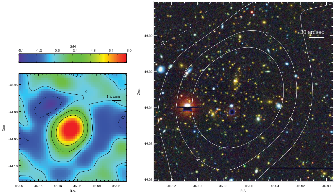
Figure 13. SPT-CL J0304-4401 at z_{rs} = 0.52 . Blanco/MOSAIC-II irg images are shown in the optical/infrared panel. (A color version of this figure is available in the online journal.)
