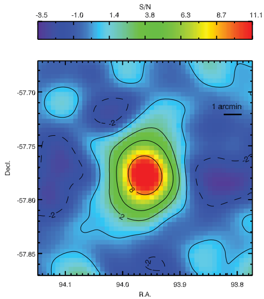
Figure 19. SPT-CL J0615-5746 at z_{\text{spec}} = 0.972 . Blanco/NEWMIR K_s and Blanco/MOSAIC-II rg images are shown in the optical/infrared panel. (A color version of this figure is available in the online journal.)
