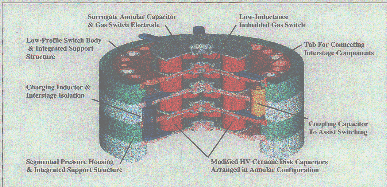
Figure 1. Cutaway-view drawing of the ultra-compact Marx showing key components and integrated packaging.
