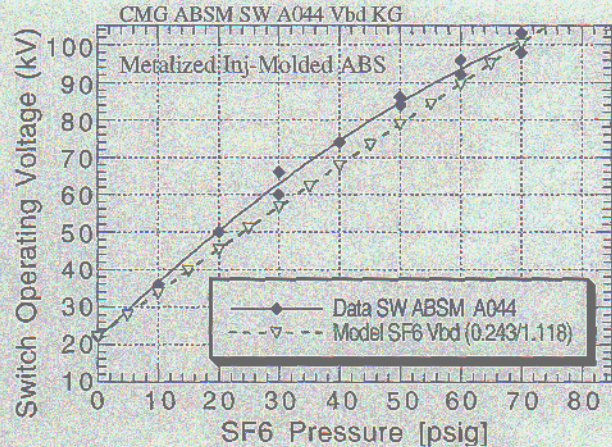
Figure 4. Operating curve of miniature gas switch.
