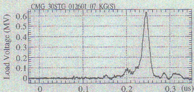
Figure 10. Output voltage into 50 ohm resistive load
