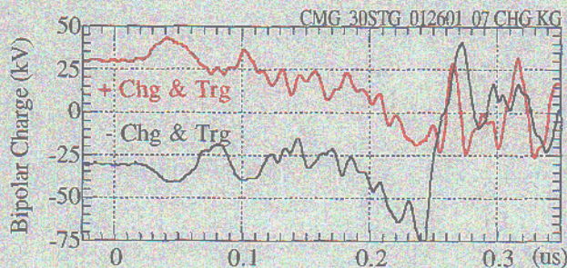
Figure 9. Voltage on charge lines during triggering.
