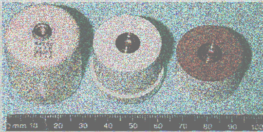
Figure 2. Modifications to commercial disk capacitors.
