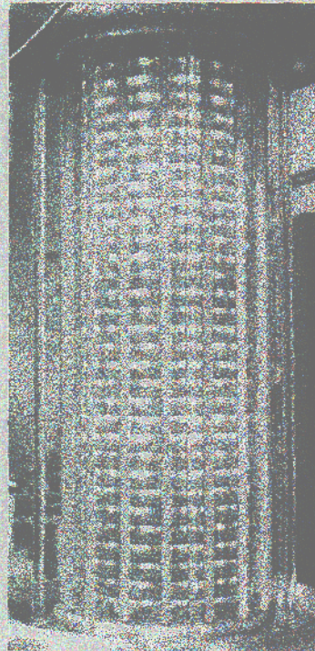
Figure 8. Photograph of 30-stage Ultra-Compact Marx during operation
