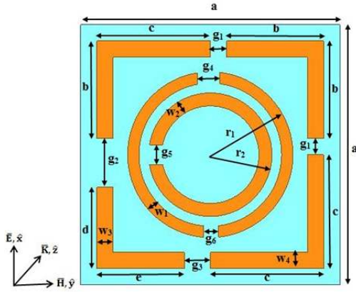
Fig. 1. Top layer of the proposed unit cell structure.
