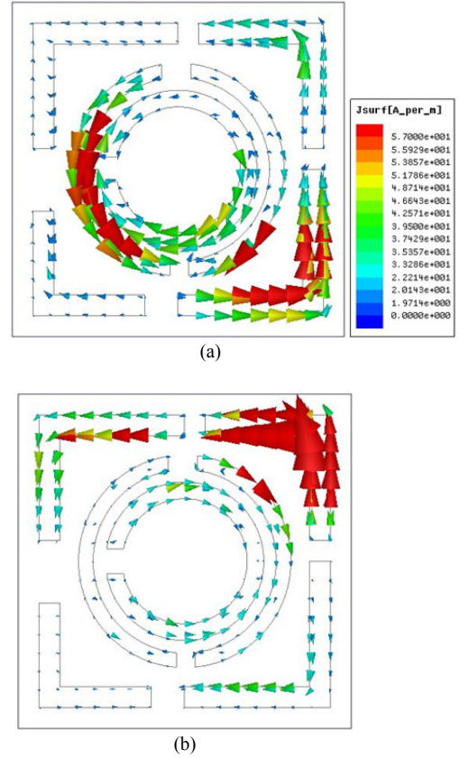
Fig. 8. Surface current distributions on top layer at (a) 13.2 GHz and (b) 16.5 GHz.
