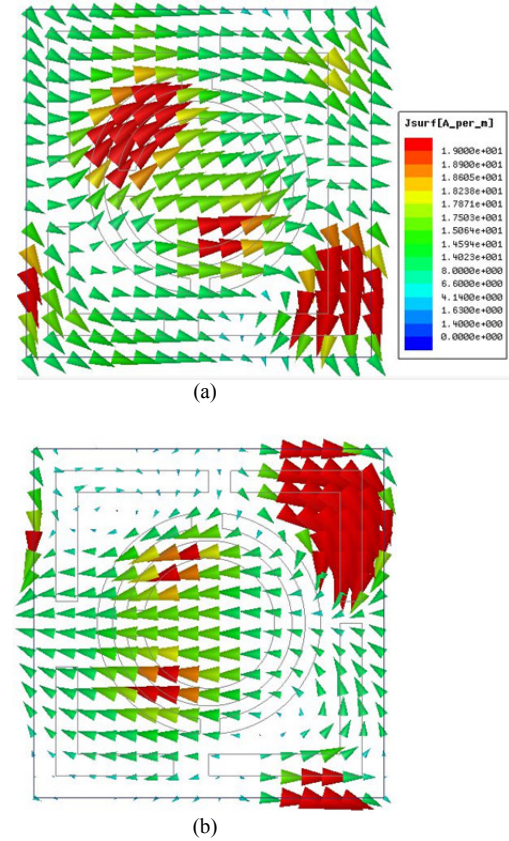
Fig. 9. Surface current distributions on bottom layer at (a) 13.2 GHz and (b) 16.5 GHz.
