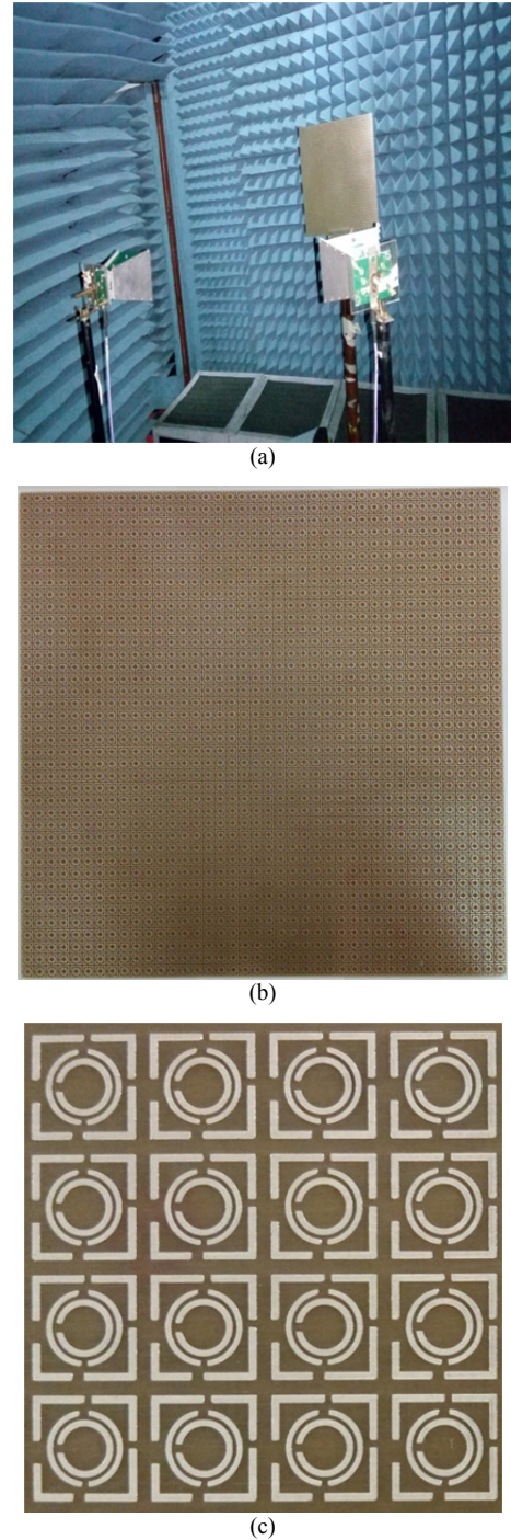
Fig. 11. (a) The experimental set up and (b) the fabricated absorber, with (c) the enlarged view.
