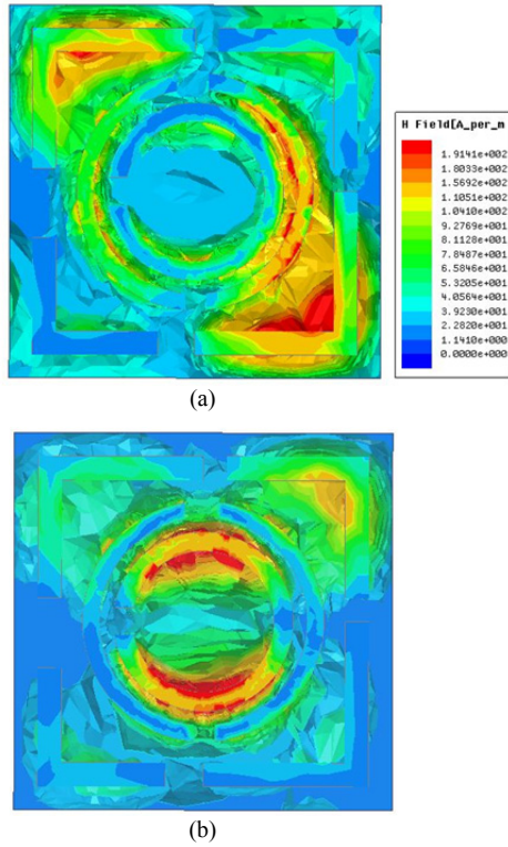
Fig. 7. Magnetic field distributions at (a) 13.2 GHz and (b) 16.5 GHz.
