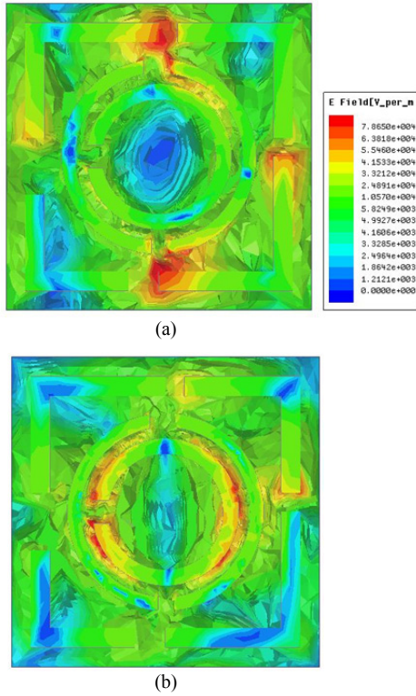
Fig. 6. Electric field distributions at (a) 13.2 GHz and (b) 16.5 GHz.
