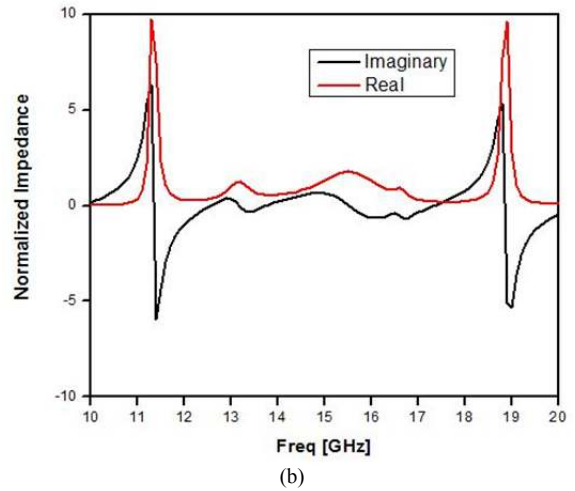
Fig. 2. (a) Simulated absorptivity and (b) normalized impedance.
