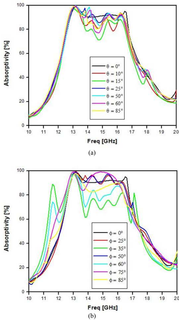
Fig. 10. Simulated absorptivities under (a) oblique and (b) normal incidence for TE polarization.
