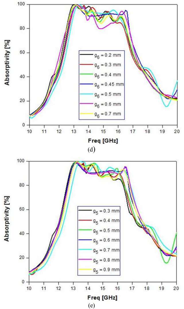
Fig. 5. Simulated absorptivities under variations of (a), (b) widths and (c), (d), (e) gaps of the of the circular split rings.
