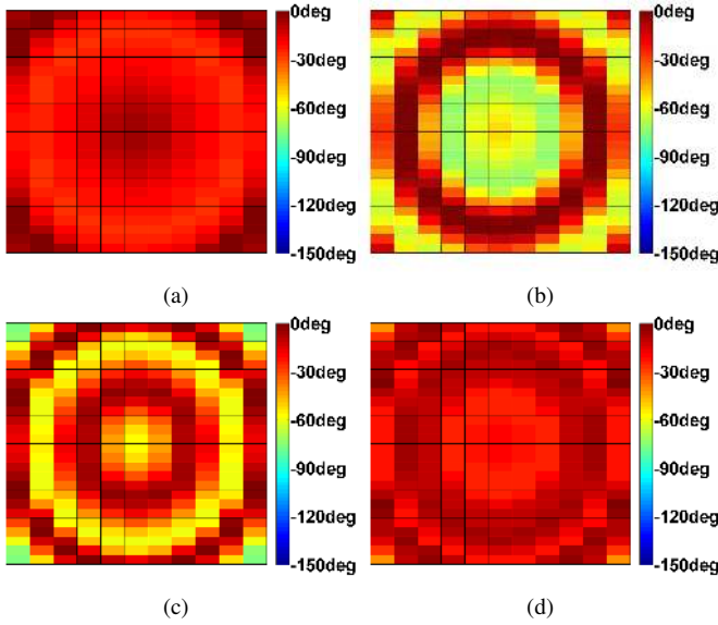
Fig. 8. Phase error distribution at (a) 4 GHz, (b) 7 GHz, (c) 9 GHz and (d) 10 GHz when d(l_1) is used to design the reflectarray.
