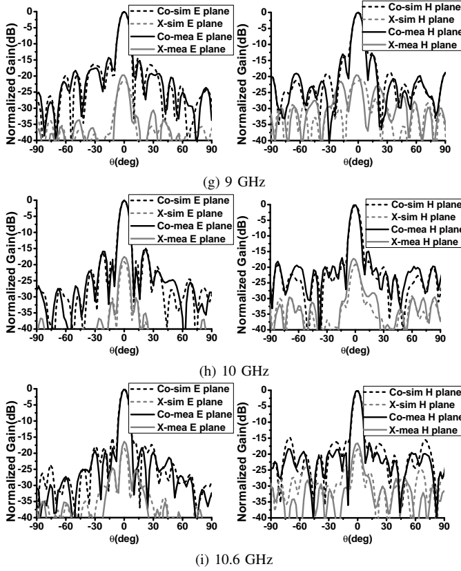
Fig. 13. Radiation patterns of the TCDR.
