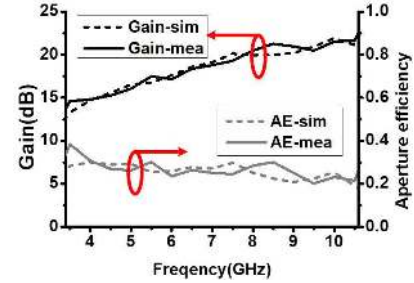
Fig. 16. Simulated and measured gains and aperture efficiency.
