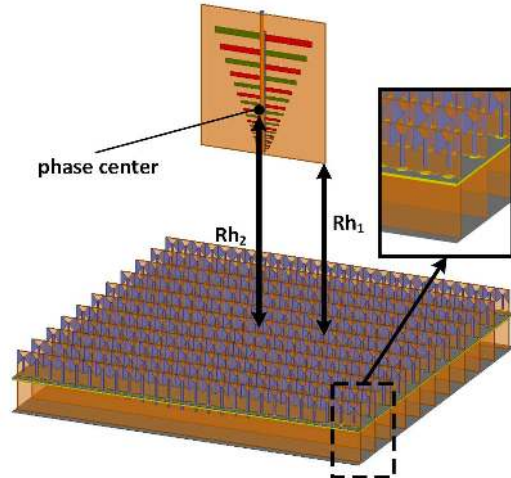
Fig. 7. Configuration of the TCDR antenna.
