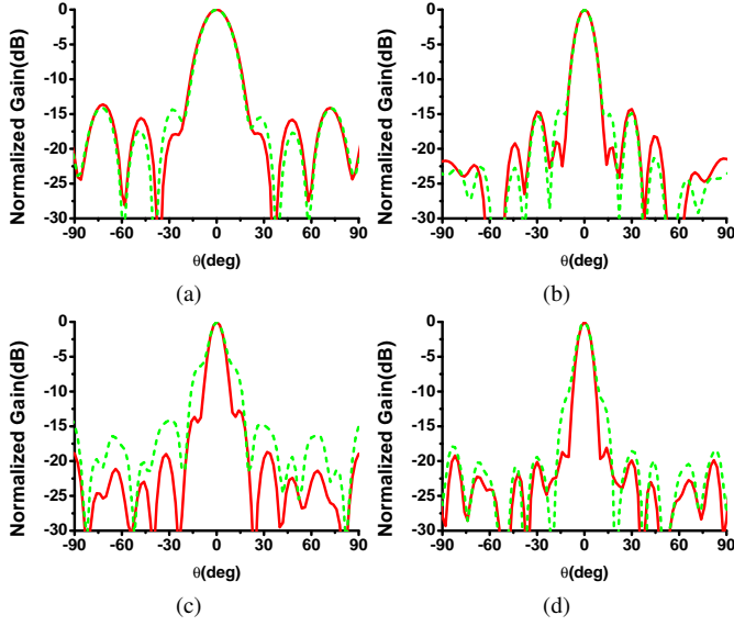
Fig. 11. Simulated radiation patterns at (a) 4 GHz, (b) 7 GHz, (c) 9 GHz and (d) 10 GHz when d(l_1) and d_{7GHz}(l_1) are used to design the reflectarray respectively. Solid lines are patterns when d(l_1) is used. Dash lines are patterns when d_{7GHz}(l_1) is used.
