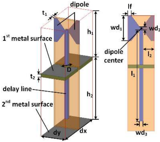
Fig. 2. Side and front views of the proposed element.
