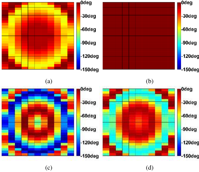
Fig. 9. Phase error distribution at (a) 4 GHz, (b) 7 GHz, (c) 9 GHz and (d) 10 GHz when d_{7GHz}(l_1) is used to design the reflectarray.
