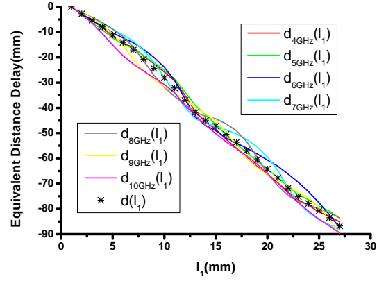
Fig. 3. Equivalent distance delay of the proposed element.
