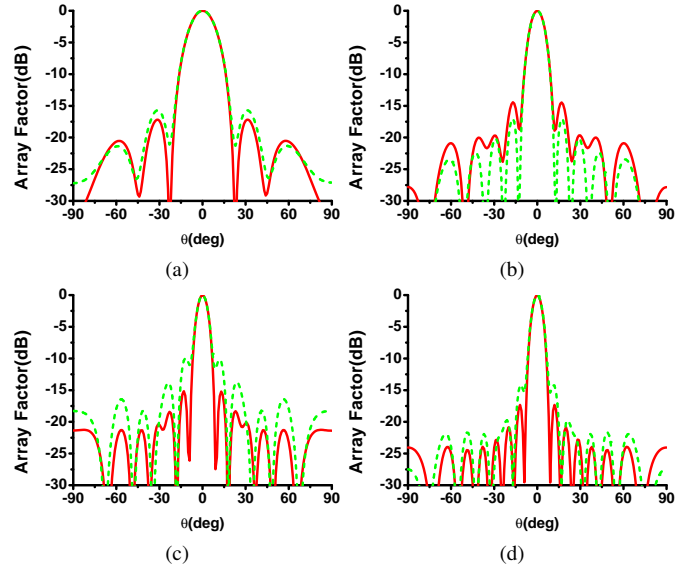
Fig. 10. Array factors at (a) 4 GHz, (b) 7 GHz, (c) 9 GHz and (d) 10 GHz when d(l_1) and d_{7GHz}(l_1) are used to design the reflectarray respectively. Solid lines are array factors when d(l_1) is used. Dash lines are array factors when d_{7GHz}(l_1) is used.
