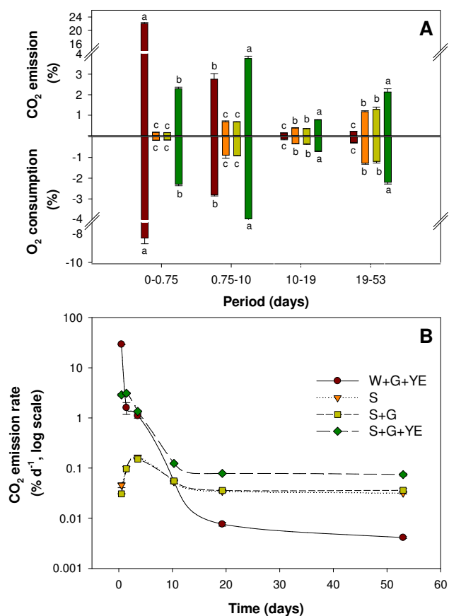
Fig. 3. (A) Total (labelled + unlabelled) CO 2 emission and O 2 consumption from irradiated-soil ( S ); irradiated-soil + labelled glucose ( S + G ); irradiated-soil + labelled glucose + yeast-extract ( S + G + YE ); water + labelled glucose + yeast-extract ( W + G + YE ) for four periods of incubation. Results are expressed as % of microcosm atmosphere. Water with labelled glucose was also incubated as control, but CO 2 emission from this control was null and not reported. Letters at each sampling date indicate the ANOVA-based differences at 5 % P-level among treatments. (B) Total (labelled + unlabelled) CO 2 emission rate from water and soil microcosms. Symbols are the same as Fig. 3a.
