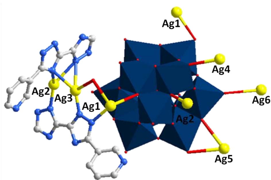
Fig.S1 Combined polyhedral and ball/stick representation of the molecular structure unit of 1 .
