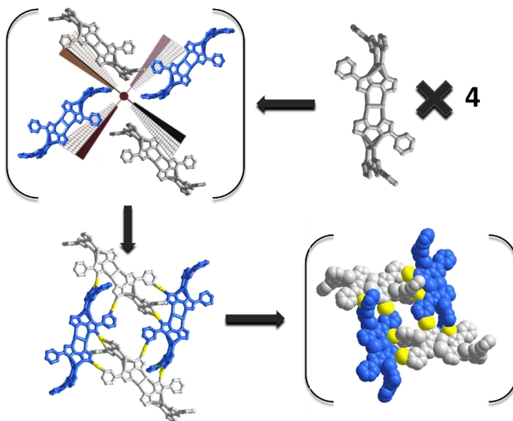
Fig. S3 Ball/stick/space representation of “windmill-like” TMC
