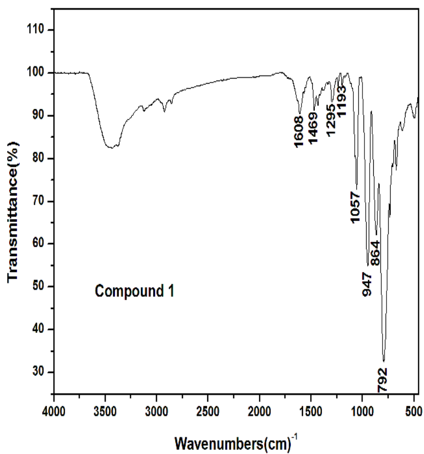
Fig.S5 The IR spectrum of compound 1 .
