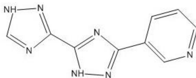
Scheme S1 The structure of pyttz ligand.
