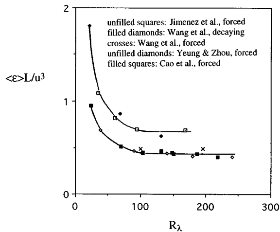
FIG. 1. The variation of the quantity \langle \epsilon \rangle L / u^3 with the Taylor microscale Reynolds number, R_\lambda , in simulations of homogeneous and isotropic turbulence in periodic box. The symbols, described on the figure, correspond to different sources of data noted in Table I.
