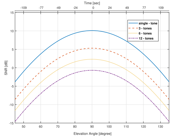
FIGURE 19. Link budget as a function of satellite elevation angle and time.
