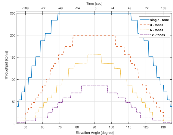
FIGURE 22. Cell NPUSCH achievable data.
