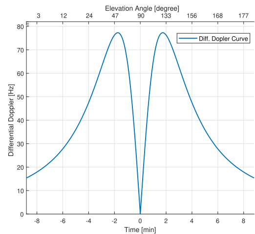
FIGURE 7. Maximum differential Doppler curves along y-axis.
