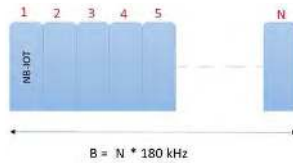
FIGURE 10. Needed resources in the uplink transmission.
