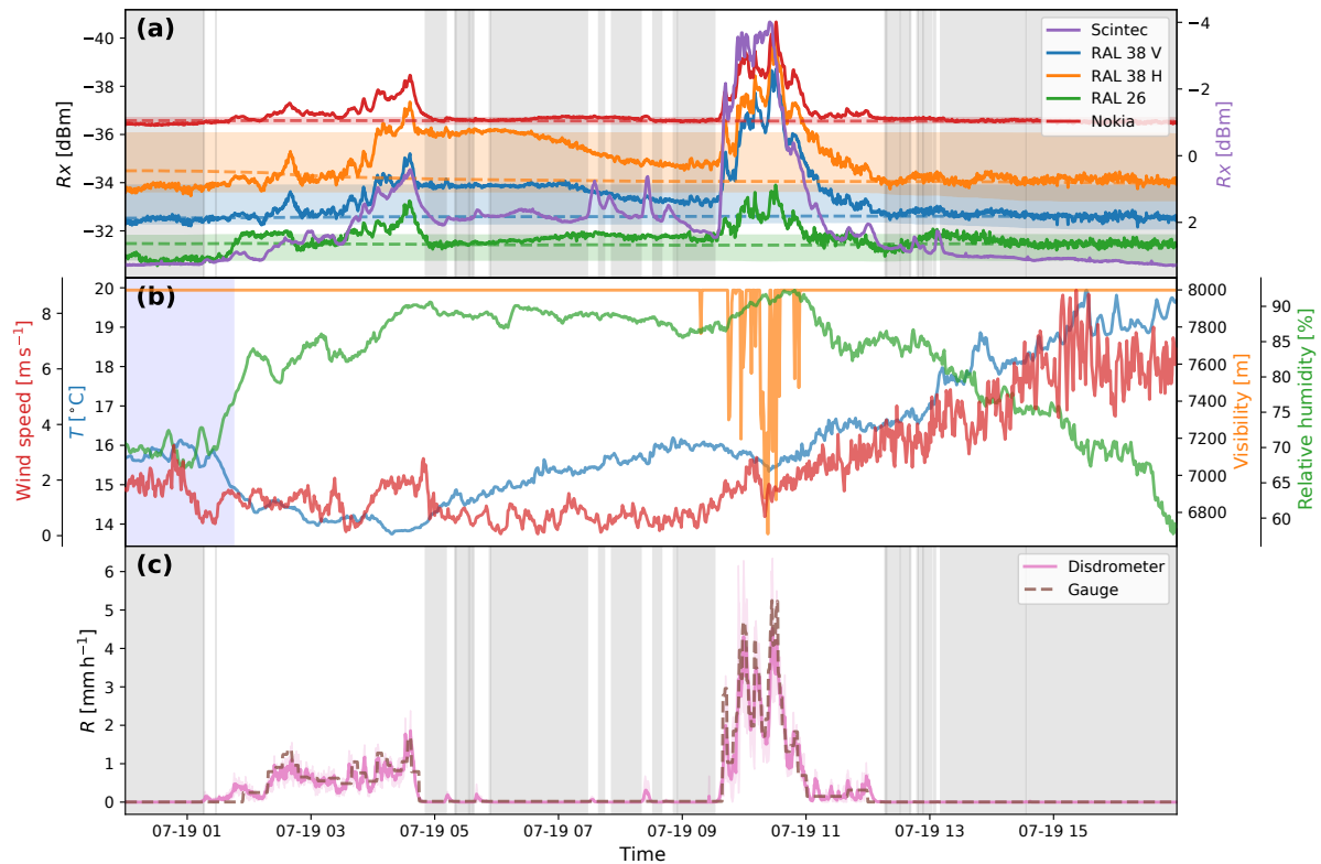
Figure 16. Time series of an event on 19 July 2015. (a) Received power levels at the detectors (solid lines) and reference levels (median over dry periods in a 24 h moving window: dashed lines). The 5th and 95th percentile power levels over dry periods in a 24 h moving window are indicated by the coloured shading. (b) Several atmospheric variables measured at the “Veenkampen” meteorological station: relative humidity, visibility, and ambient air temperature at 2 m, and wind speed indicated with blue, orange, green, and red lines, respectively. Periods with a negative net radiation flux at the surface are indicated with blue shading. (c) The spatial weighted average rainfall intensities derived from the disdrometers are indicated by the pink line, with the weighted standard deviation among the disdrometers displayed by the pink shaded area. The rainfall intensities derived from the tipping bucket gauge are indicated with the dashed line. Dry periods, as indicated by the disdrometers, are displayed by grey shaded areas.
