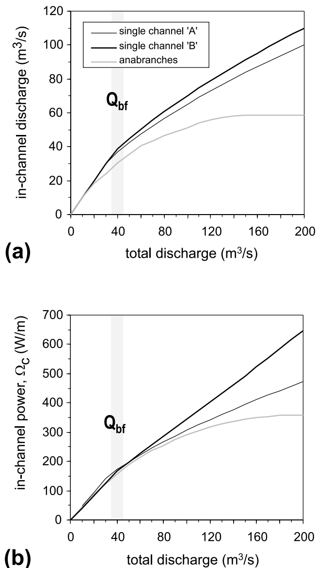
Figure 7. (a) In-channel discharge relative to total discharge in the anabranches and single channels “A” and “B” and (b) in-channel power ( \Omega_c ) relative to total discharge. In-channel discharge was calculated as the velocity-area product using the mean section method, total discharge was calculated from the GS-8210009 rating curve, and power was calculated from equation (1) using field-measured water slopes.
