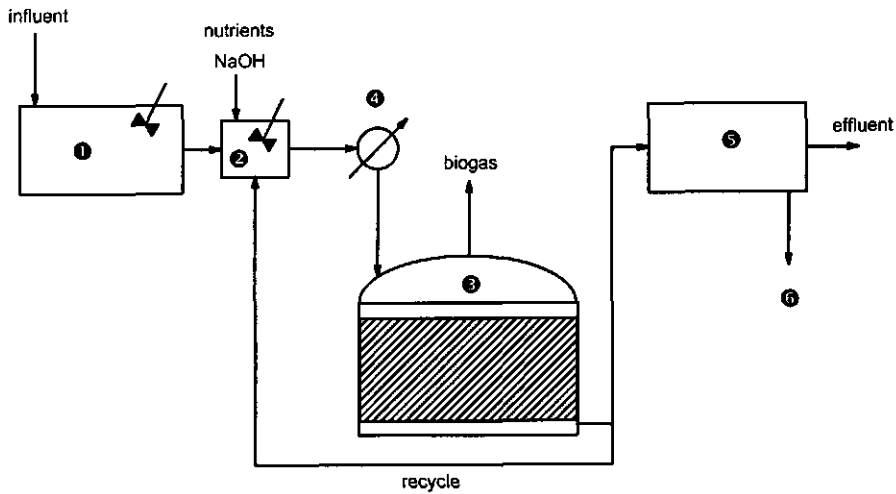
Figure 1.13: Flow sheet of the anaerobic-aerobic wastewater treatment plant for the terephthalic acid and isophthalic acid production plant from Amoco, at Geel, Belgium. The anaerobic bioreactor is a down-flow fixed-film reactor (DFF) with a volume of 15,000 m 3 . Operational data are described in the text [26]. Numbers stand for ① buffer tank ② conditioning tank, ③ anaerobic down-flow fixed-film reactor, ④ heat exchanger, ⑤ aerobic post-treatment, ⑥ sludge treatment. The picture above the flow sheet shows the two anaerobic (background) and aerobic (foreground) reactors constructed by Amoco in Kaohsiung, Taiwan.
