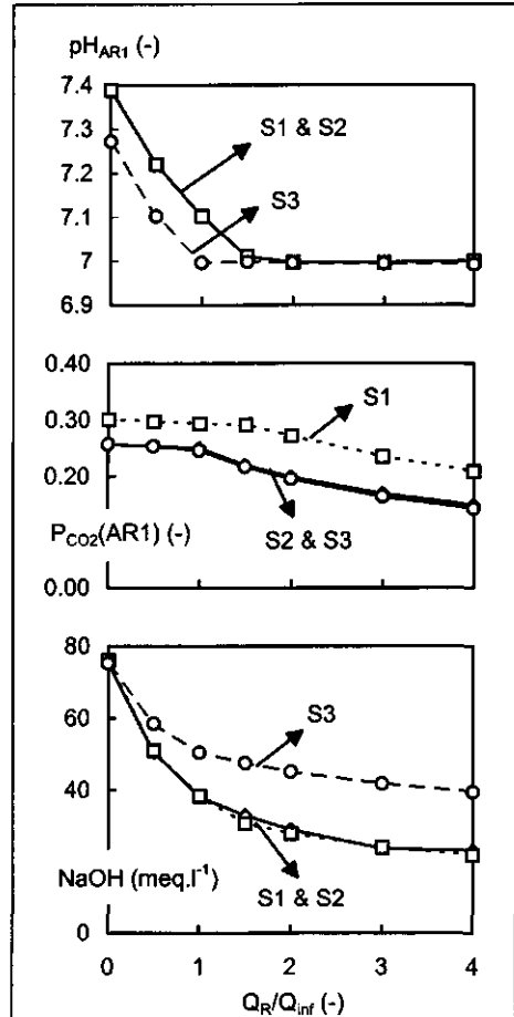
Figure 8.6: Influence of recirculation on the sodium hydroxide requirements for neutralisation (bottom graph), the \text{CO}_2 partial pressure in AR1 (middle graph) and the pH in AR1 (top graph). Boundary conditions and definitions are explained in Figure 8.4.
