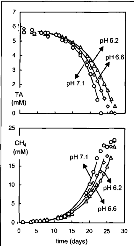
Figure 6.4: Terephthalate (TA, top graph) degradation and concomitant methane ( \text{CH}_4 , bottom graph) production by biomass from R37 at three different pH-values. Drawn lines were calculated using an equal initial volumetric conversion rate and the maximum specific growth rates shown in figure 5.
