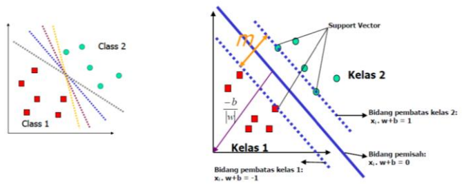
Gambar 1. Hyperplane Support Vector Machine [12]
