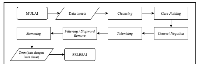
Gambar 3. Alur Proses Data Preprocessing
