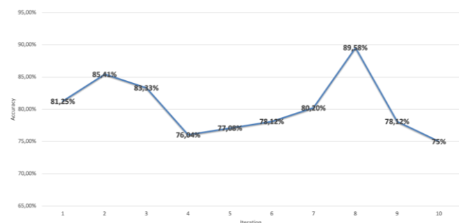
Gambar 6. Hasil 10-fold Cross Validation
