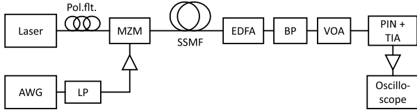
Figure 3 Experimental setup
