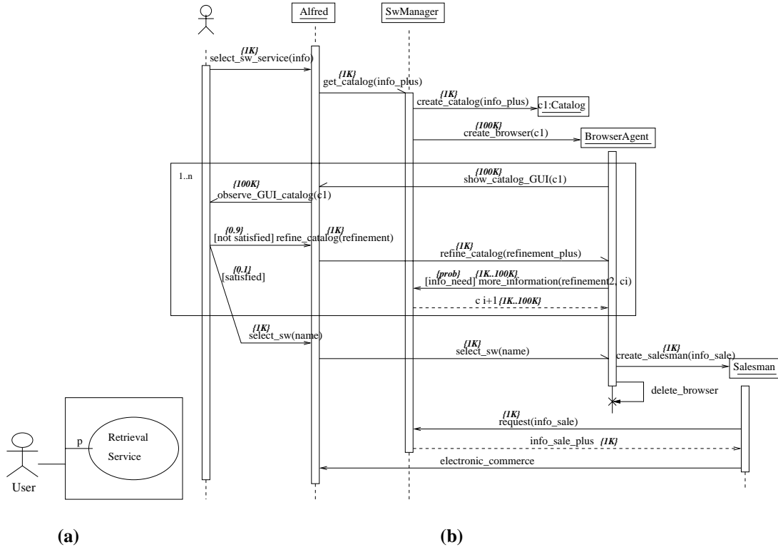
Figure 6: (a) Use case for the ANTARCTICA SRS and (b) annotated sequence diagram for the retrieval service use case.
