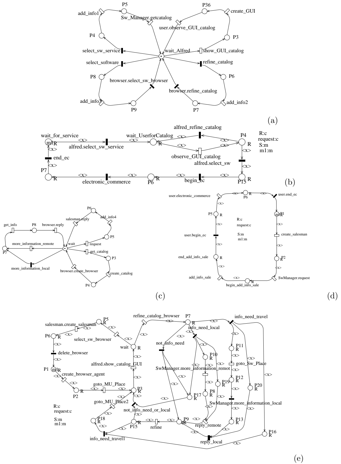
Figure 8: Component PN for the ANTARCTICA SRS: (a) Alfred, (b) user, (c) software manager, (d) salesman and (e) browser.
