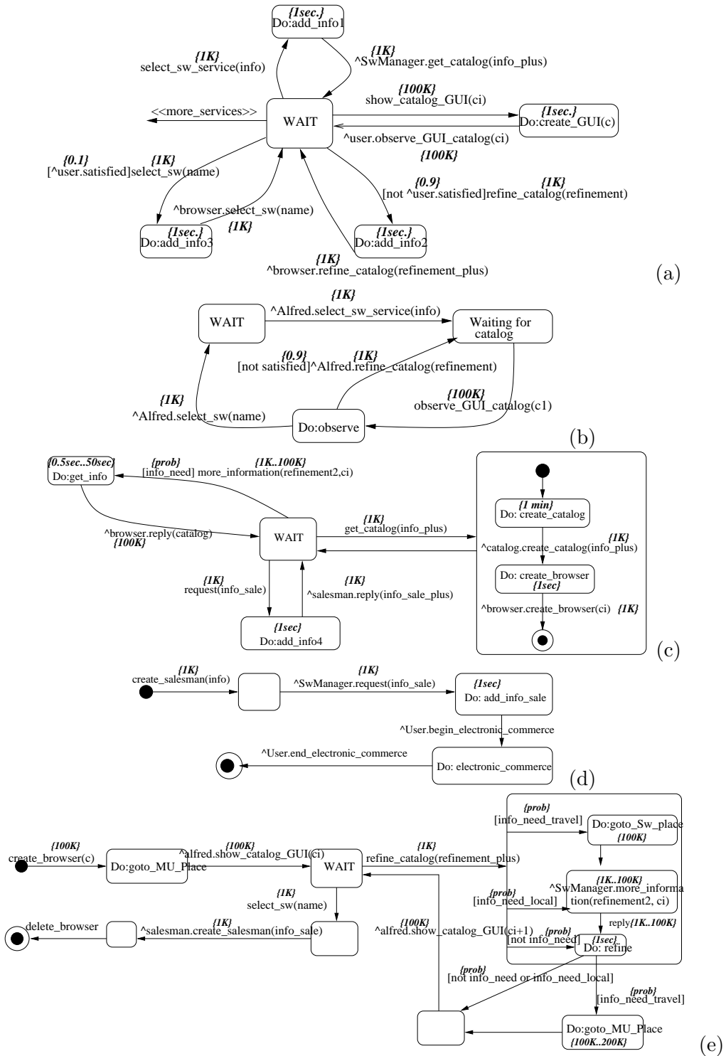
Figure 7: Annotated statecharts for the ANTARCTICA SRS: (a) Alfred, (b) user, (c) software manager, (d) salesman and (e) browser.
