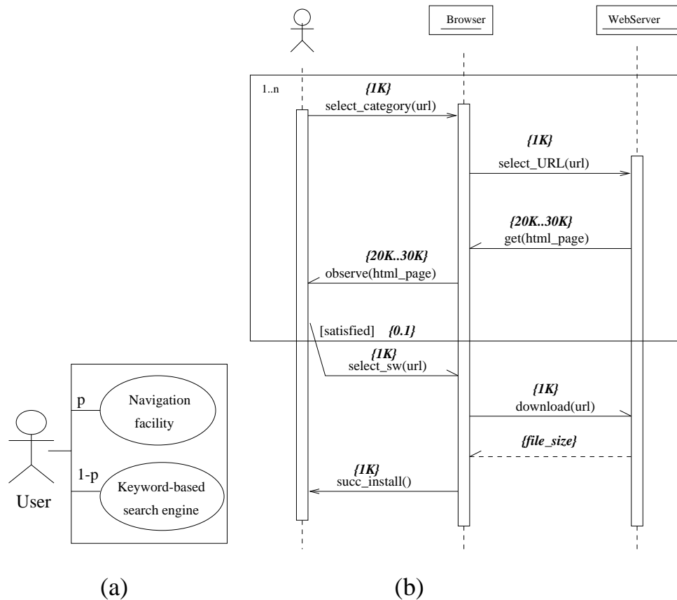
Figure 1: (a) Use cases for the Tucows-like system and (b) annotated sequence diagram for the navigation facility use case.
