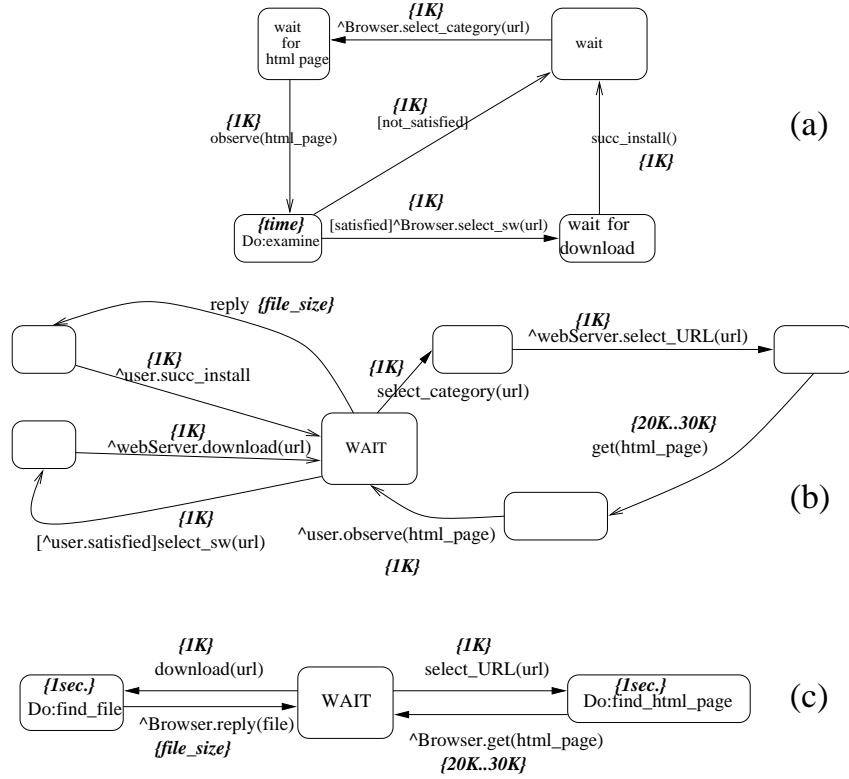
Figure 2: Annotated statecharts for Tucows-like system: (a) user, (b) browser, and (c) the web server.
