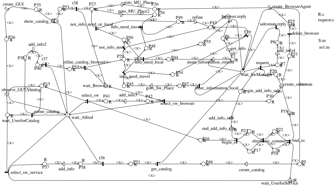
Figure 9: Complete SWN for the ANTARCTICA SRS.
