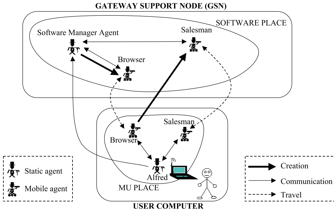
Figure 5: Architecture for the ANTARCTICA SRS.
