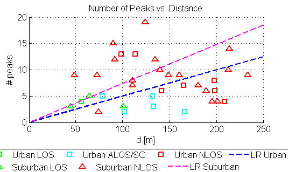
Fig. 7. Number of peaks detected vs. distance and propagation conditions.
