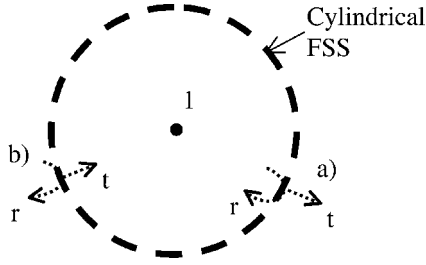
Fig. 1. Characteristics of a cylindrical FSS: (a) reflection and transmission coefficients for a cylindrical wave coming from inside to outside, (b) reflection and transmission coefficients for a cylindrical wave coming from outside to inside.
