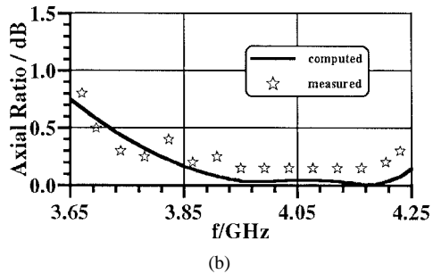
Fig. 5. Measured and computed performance of a four-section C -band septum polarizer [cf. Fig. 1(b)]; ridge thickness t/a = 0.035 . Measurements include transitions to rectangular waveguides at input ports.
