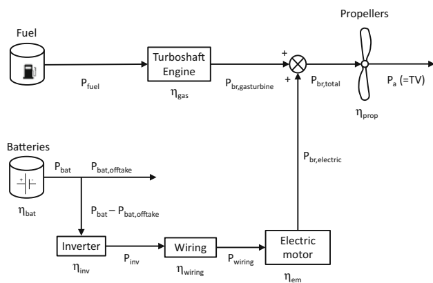
Fig. 2 Parallel hybrid electric propulsion system architecture
