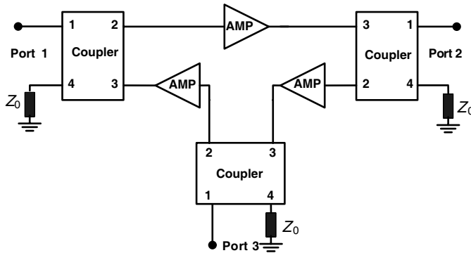
Figure 6. Basic configuration for active 3-port circulator.
