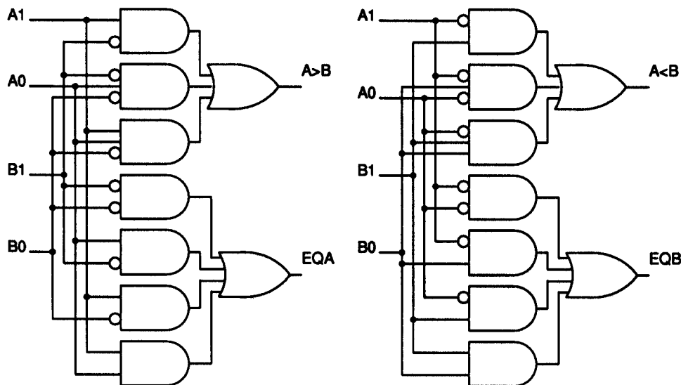
FIGURE 8 Alternate 2-bit comparator initial stage.
