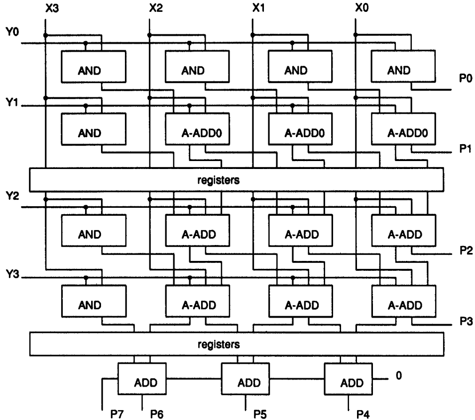
FIGURE 17 Pipelined carry save parallel multiplier implementation.
