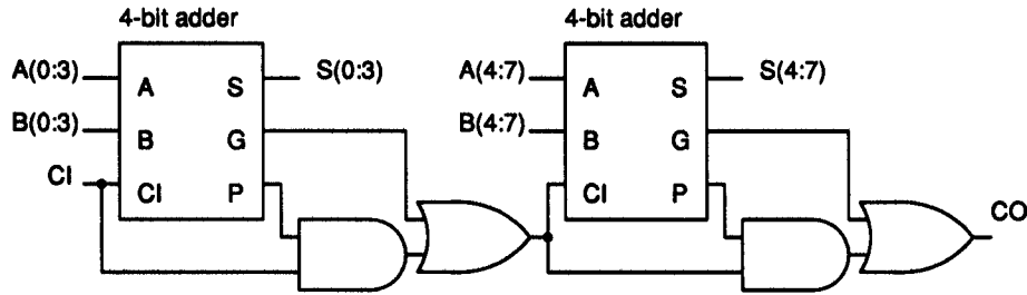
FIGURE 2 Carry bypass adder implementation.
