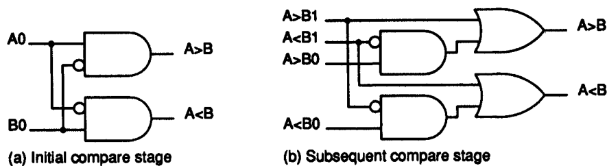
FIGURE 12 Comparator tree basic cells.
