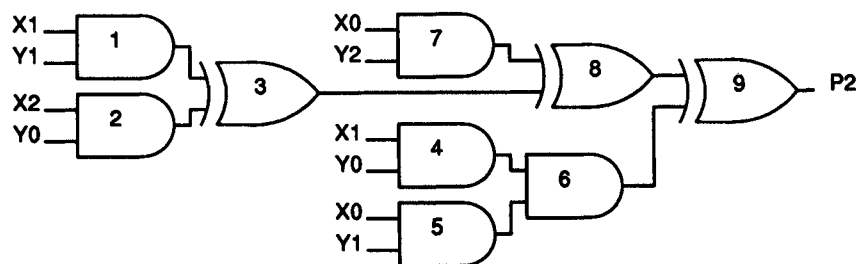
FIGURE 16 Combined logic for P2 output of carry save multiplier.
