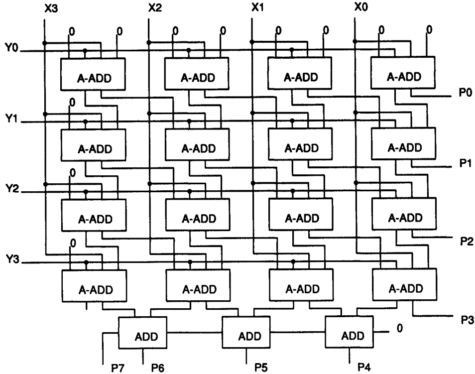
FIGURE 14 Carry save parallel multiplier implementation.
