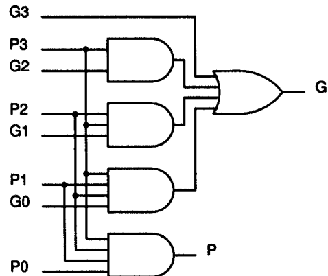
FIGURE 3 Cumulative propagate and generate implementation.
