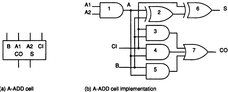
FIGURE 15 Carry save multiplier basic cell.
