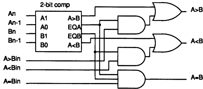
FIGURE 10 Bypass comparator.
