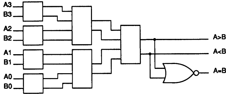
FIGURE 11 4-bit comparator tree.
