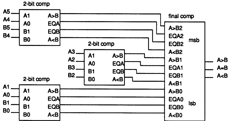
FIGURE 7 Alternate parallel comparator implementation.
