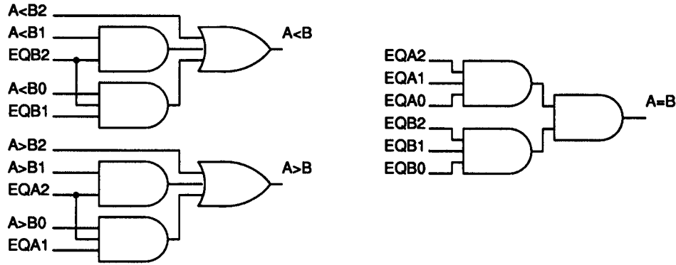
FIGURE 9 Alternate comparator final stage.
