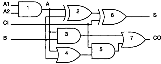
FIGURE 19 Modified carry save multiplier cell.
