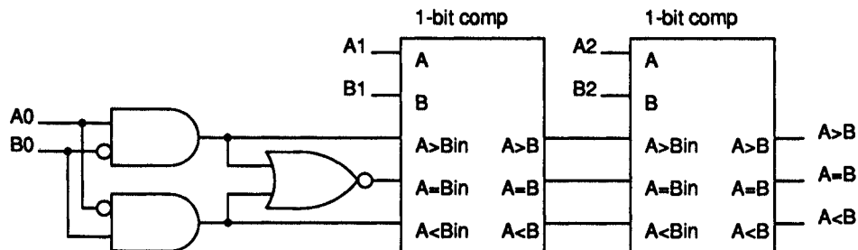
FIGURE 5 3-bit ripple comparator implementation.
