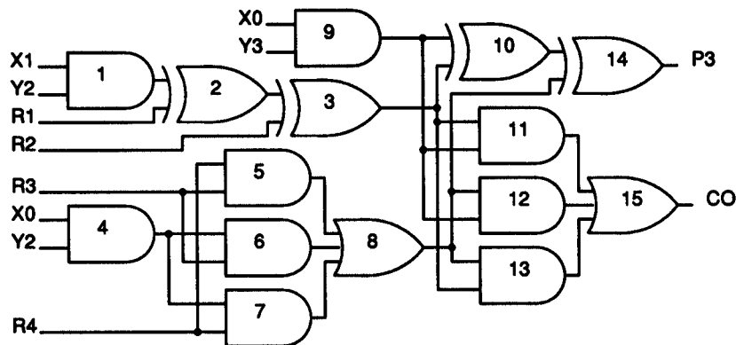
FIGURE 18 Combined logic for P_3 output of pipelined carry save multiplier.
