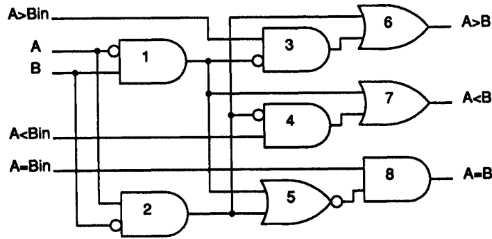
FIGURE 4 1-bit extensible comparator implementation.
