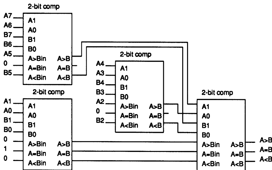
FIGURE 6 8-bit parallel comparator implementation.
