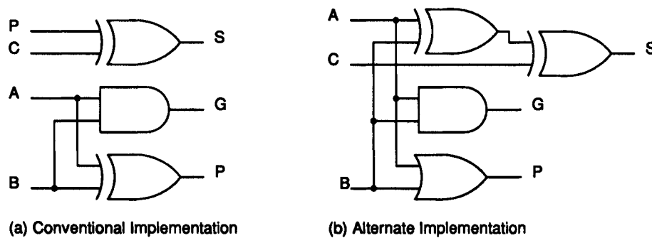
FIGURE 1 Propagate/generate logic implementation.
