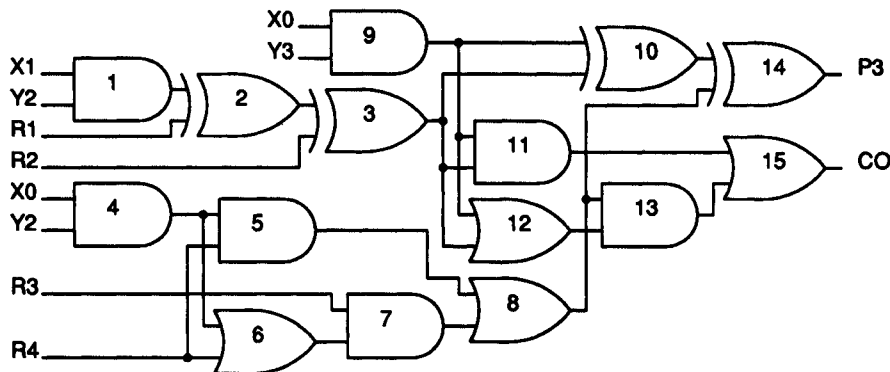
FIGURE 20 Modified logic for P3 output of pipelined carry save multiplier.
