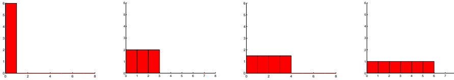
Figure 6.4: Finite time decaying functions \beta from (6.5) (a)–(d) (left to right)
