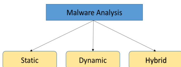
Figure 2: Malware Analysis
