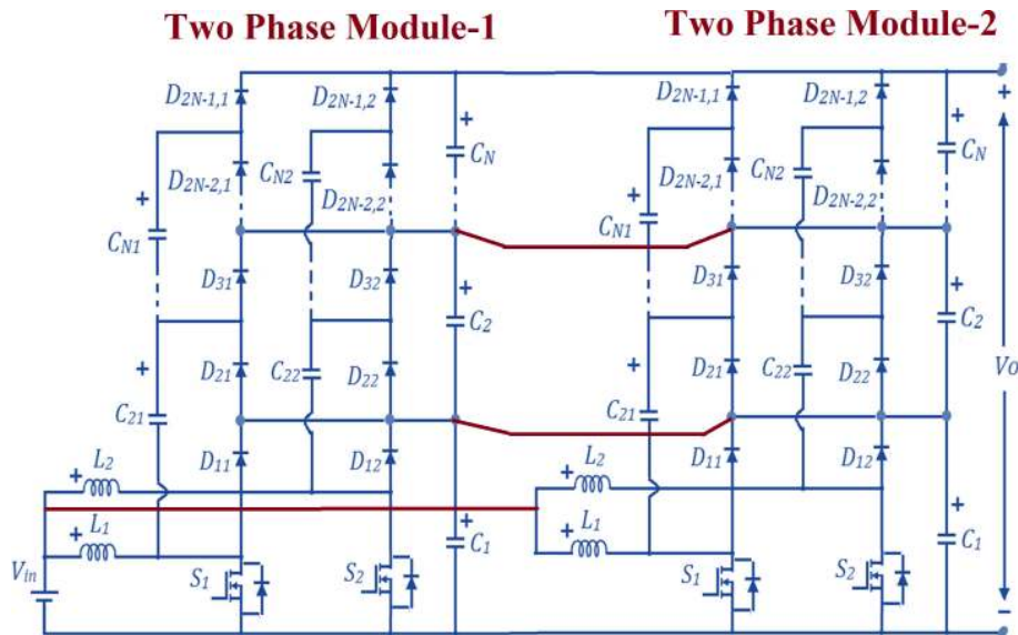
FIGURE 18. Further improvement to increase phases of the interleaved converter (four-phase of Nx IMBC).
