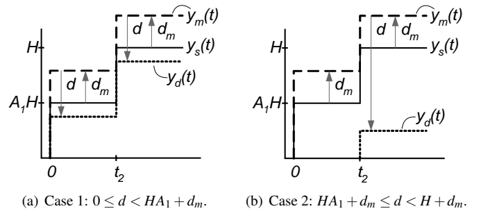
Figure 13. ZV-SHAPED STEP COMMAND MODIFIED BY DEAD-ZONE AND INVERSE-DEAD-ZONE.
