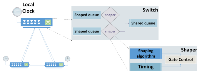
Fig. 1: Outbound architecture of ATS switch
