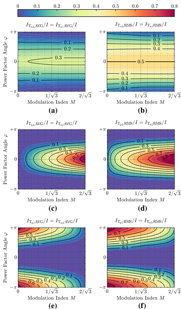
Fig. 13 Normalized I_{AVG} and I_{RMS} flowing through a, b the 2-L inverter transistors and c, d, e, f , the 3-L SM transistors, as a function of the modulation index M and the power factor angle \varphi (normalization with respect to I ). The same current values apply to the respective diodes, however the results are shifted by \varphi = \pi . The current stresses in the 2-L inverter devices are mostly independent on M , as for conventional 2-L inverters [24], while the current stresses in the 3-L SM devices strongly depend on both M and \varphi . The maximum stress in these devices is always found for \varphi = 0 or \varphi = \pi , since the average and RMS values of the current flowing into the 3-L SM (i.e. i_h ) are highest when the power transfer is maximized (i.e. \cos \varphi = \pm 1 ). Moreover, the value of M varies the conduction time intervals of the 3-L SM internal devices ( T_{p,h}, T_{n,l} ) and external devices ( T_{p,l}, T_{n,h} ), maximizing their current stresses for M = 0 and M = 2/\sqrt{3} , respectively
