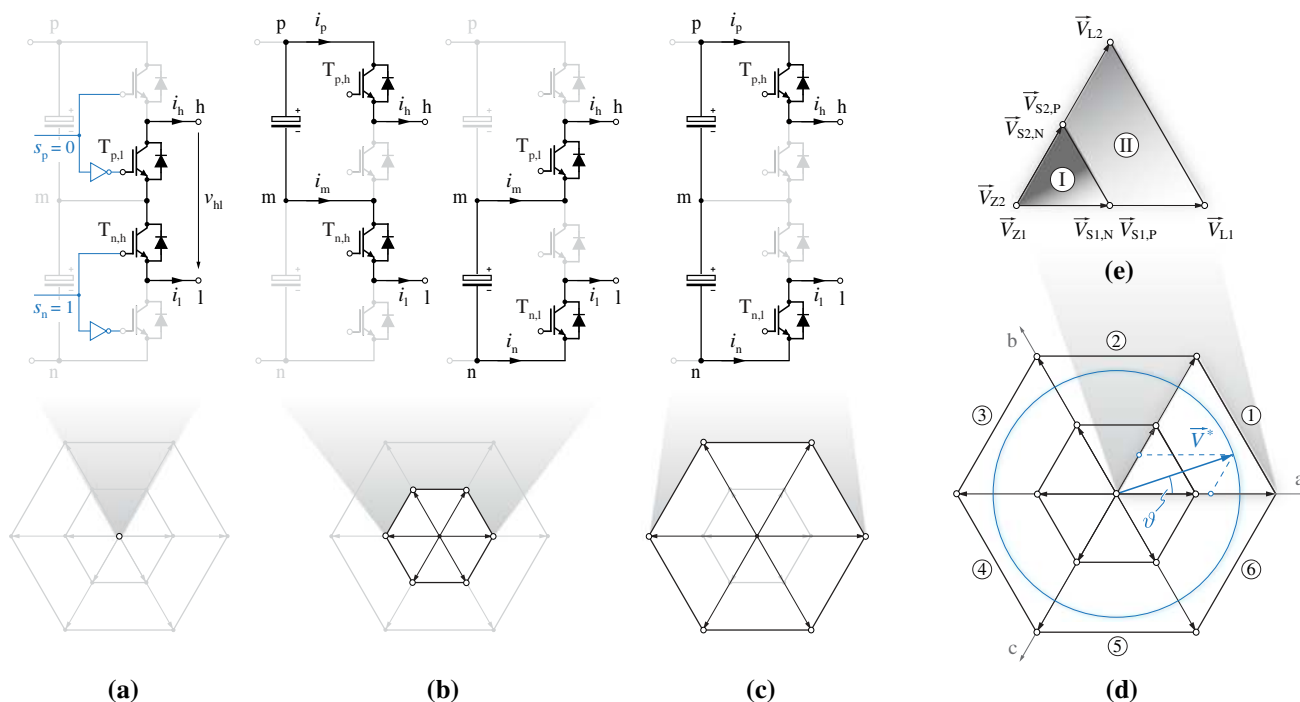
Fig. 2 Schematic of the 3-L switching matrix (SM) conduction states and respective SNPCC output voltage space vectors: a zero vector states, b small vector states and c large vector states. The complete SNPCC space vector hexagon is illustrated in (d) , together with a reference voltage vector \vec{V}^* and its decomposition. Sector ① and its subdivision in area ① and area ② are highlighted in (e) in combination with the associated zero, small and large vectors
