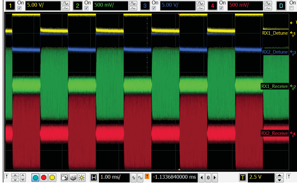
Fig. 3.17. RX load output in tight RX-RX coupling with TDM method
