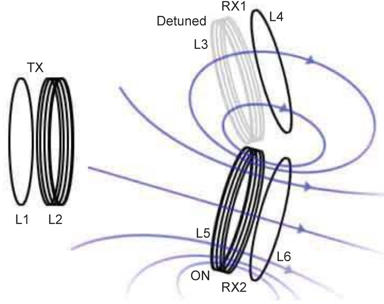
Fig. 3.10. Illustration on how synchronization is kept in detuned mode. Detuned receiver RX_1 is receiving the synchronization signal from resonant coil, L_5 of RX_2 .
