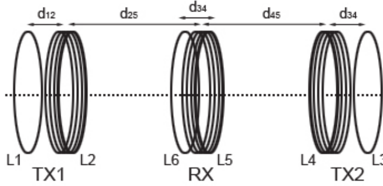
Fig. 2.10. Optimal positioning for a 2TX and 1RX experimental setup. This setup reduces coupling between transmitters while maximizing the coupling coefficient between TX and RX by having a 0^\circ angle on the same axis.
