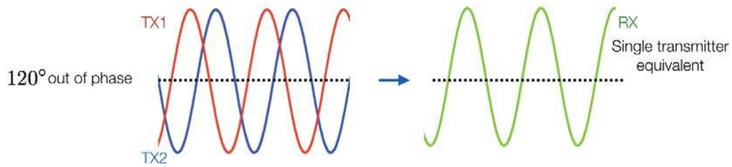
Fig. 2.5. Phase offset of 120^\circ results in an equivalent single-input single-output case in terms of received power.
