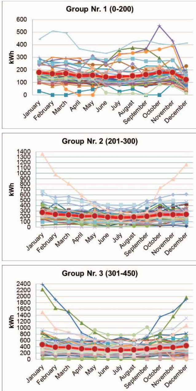
Fig. 2. Analysis of monthly electricity consumption for different consumer groups.
