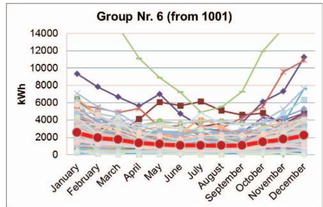
Fig. 2. Analysis of monthly electricity consumption for different consumer groups.
