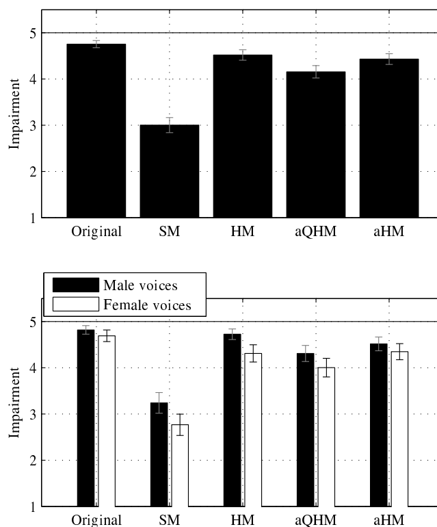
Fig. 8. Impairment evaluation of the resynthesis quality by 44 listeners using 24 utterances of 12 different languages, with the 95% confidence intervals. Global results above and gender-specific results below. The used f_0 values are those provided by the aHM-AIR method.
