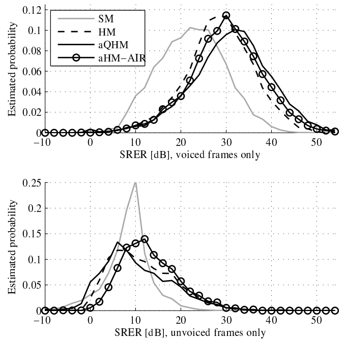
Fig. 7. Estimation of the full-band SRER distributions for voiced and unvoiced frames on top and bottom plots respectively.
