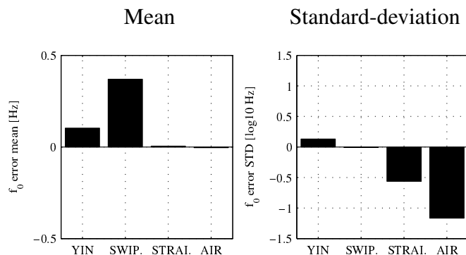
Fig. 5. f_0 error corresponding to f_0 estimation methods using the same synthetic signals as in Figure 4.
