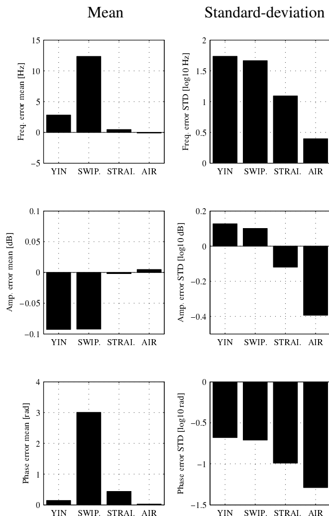
Fig. 4. Error of sinusoidal parameters according to state-of-the-art f_0 methods and the suggested f_0 refinement method AIR (computed on the full-band of the signal).
