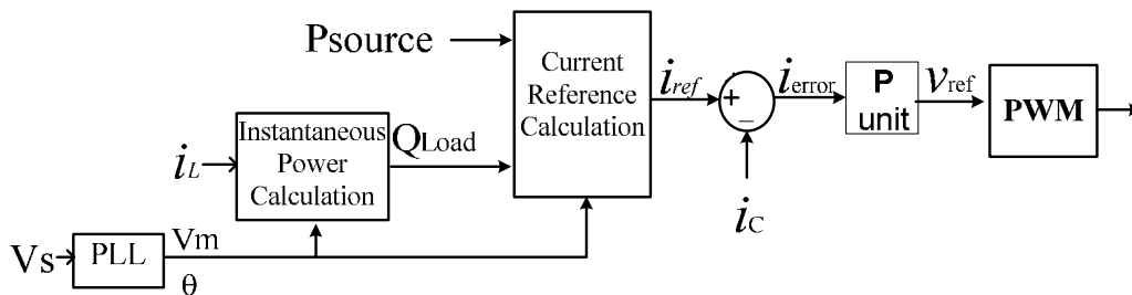
Fig. 6 Block diagram of CGCI control system
