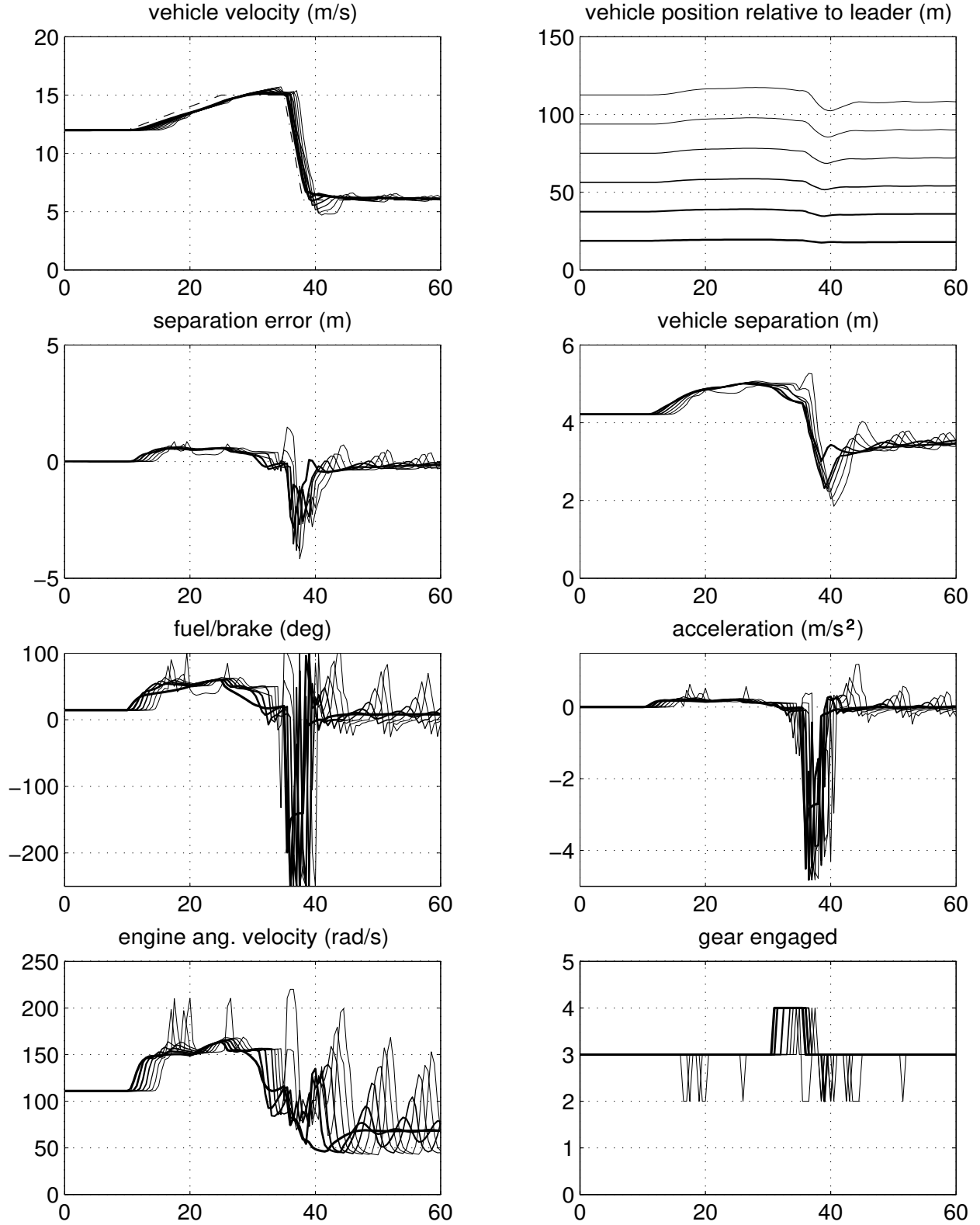
Figure 40: Actuator delay \tau = 0.2 s, backstepping controller with Smith predictor variable time headway h = 0.1 - 0.2v_r s, and variable separation error gain k = 0.1 + (1 - 0.1)e^{-0.1\delta^2} .
