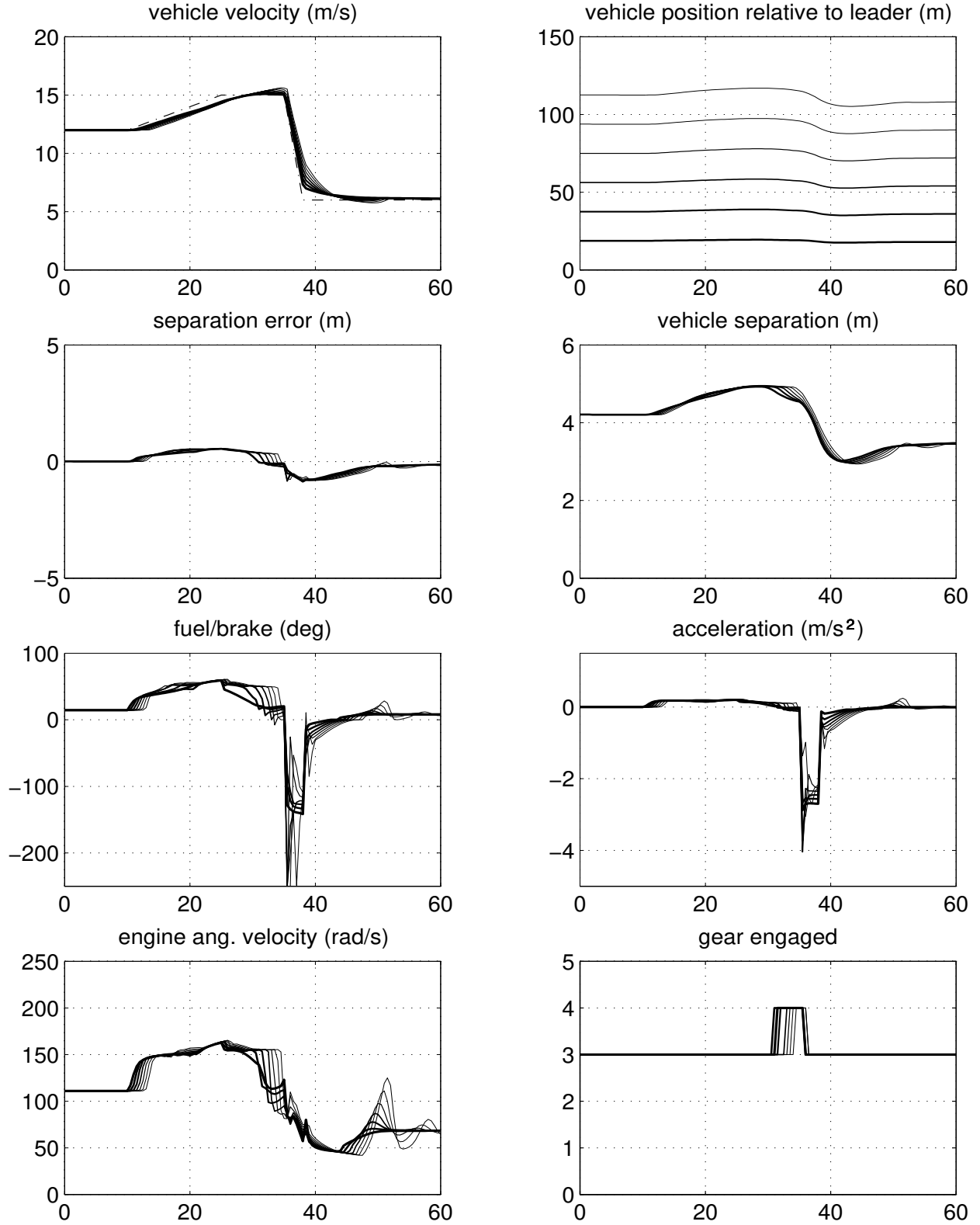
Figure 37: No delay, backstepping controller with variable time headway h = 0.1 - 0.2v_r s and variable separation error gain k = 0.1 + (1 - 0.1)e^{-0.1\delta^2} .
