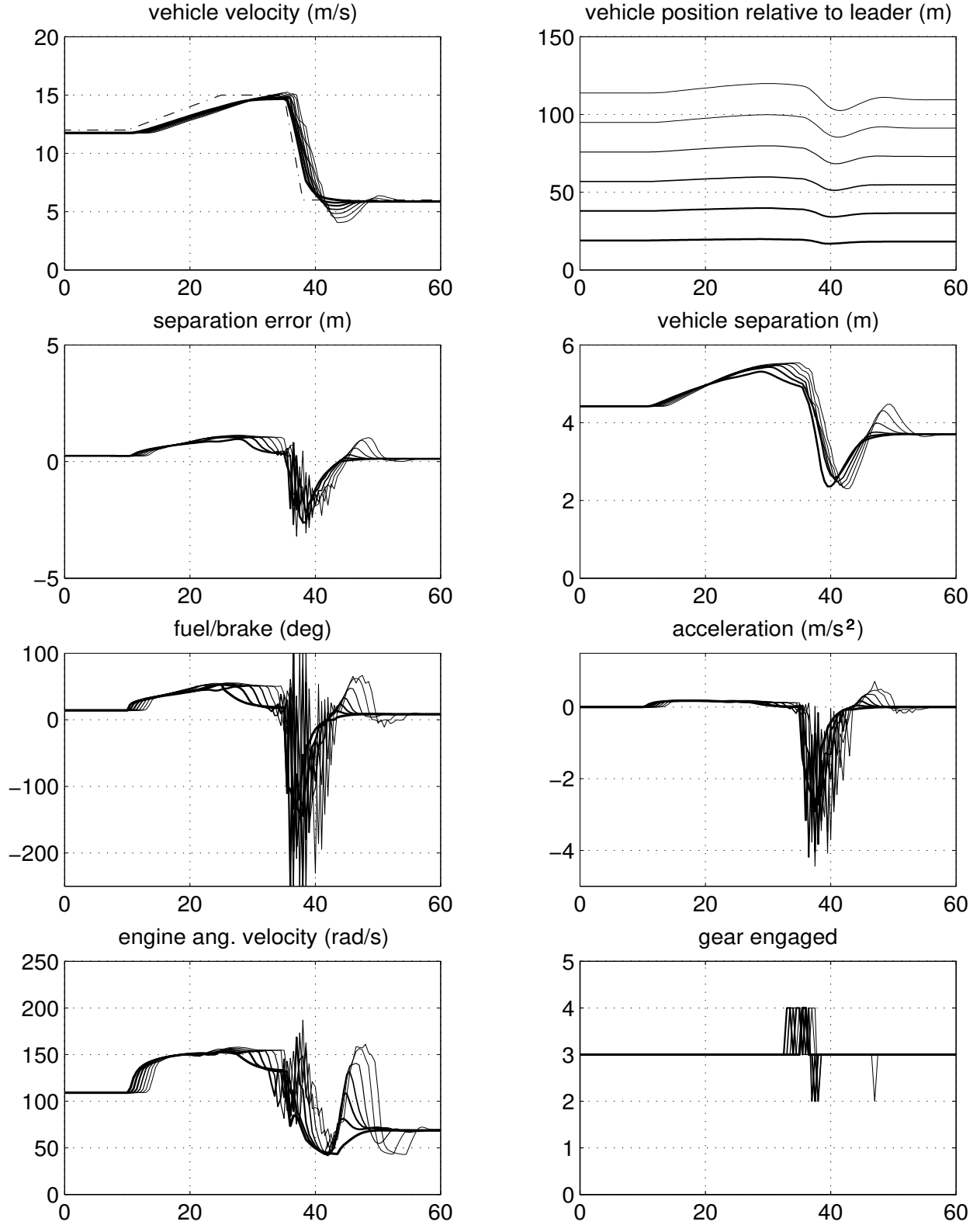
Figure 44: Actuator delay \tau = 0.2 s, PID controller, variable time headway h = 0.1 - 0.2v_f s, and variable separation error gain k = 0.1 + (1 - 0.1)e^{-0.1\delta^2} .
