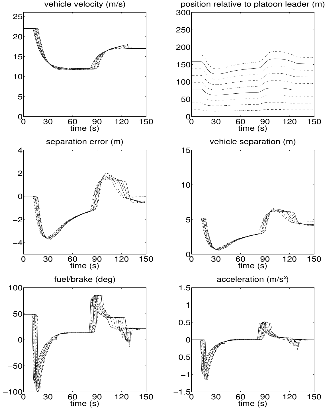
Figure 10: Ten autonomous vehicles, h = 0.1 s, variable k , \sigma = 50 .
