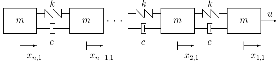
Figure 20: Mass-spring-damper system.
