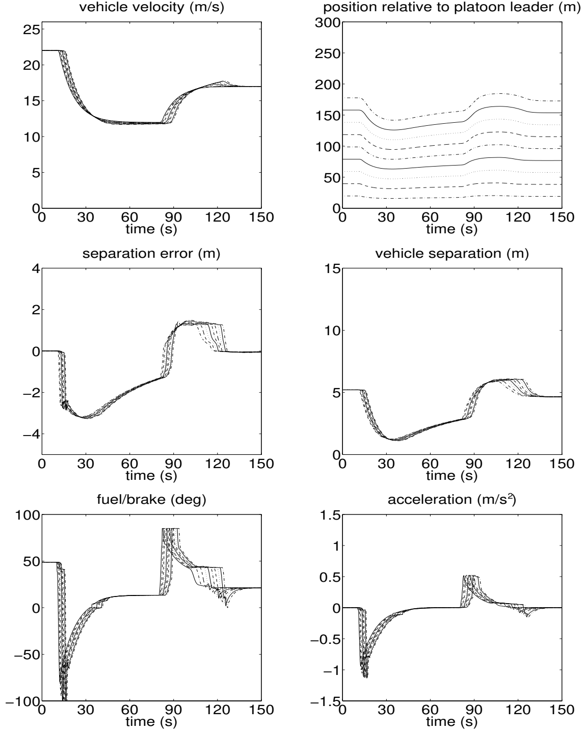
Figure 11: Ten autonomous vehicles, h = \text{sat}(0.1 - 0.2v_r) , variable k , \sigma = 50 .
