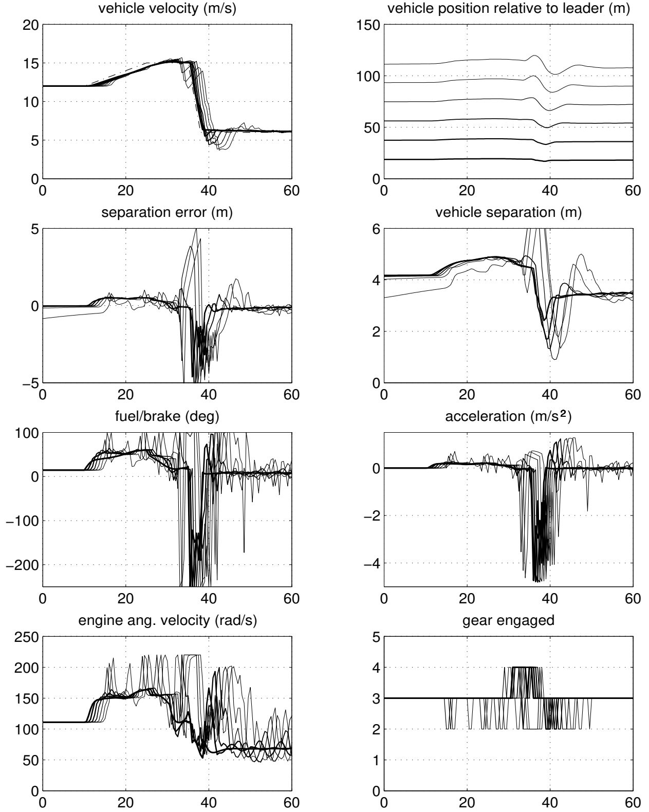
Figure 42: Actuator delay \tau = 0.3 s, backstepping controller, variable time headway h = 0.1 - 0.2v_r s, and variable separation error gain k = 0.1 + (1 - 0.1)e^{-0.1\delta^2} .
