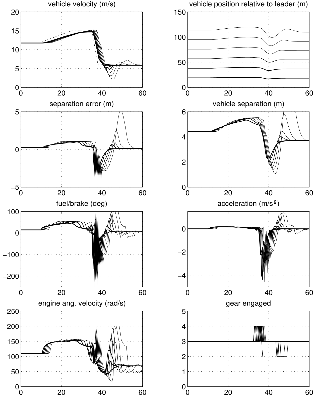
Figure 46: Actuator delay \tau = 0.3 s, PID controller, variable time headway h = 0.1 - 0.2v_f s, and variable separation error gain k = 0.1 + (1 - 0.1)e^{-0.1\delta^2} .
