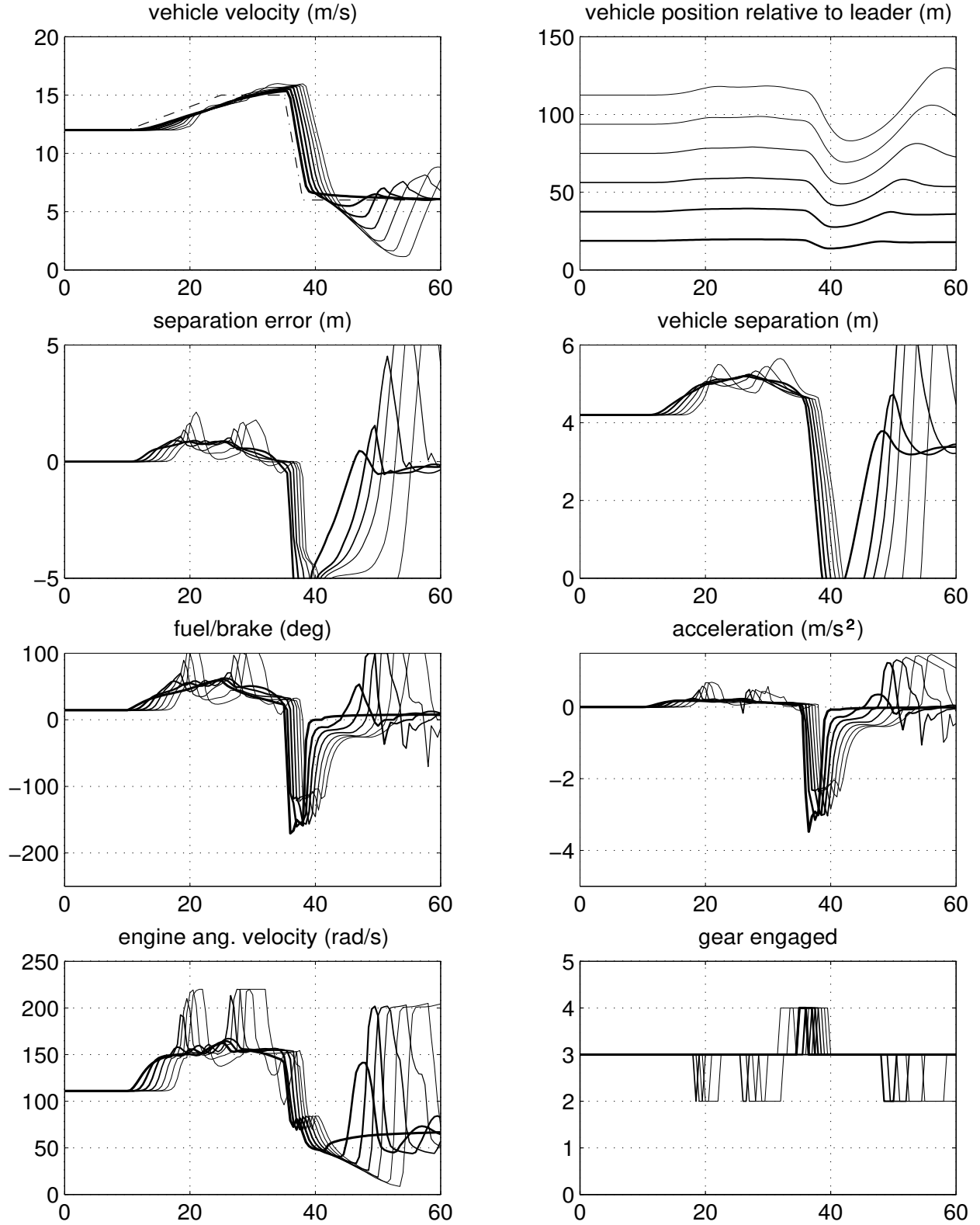
Figure 33: Actuator delay \tau = 0.2 s, original PIQ controller with variable time headway h = 0.1 - 0.2v_r s and variable separation error gain k = 0.1 + (1 - 0.1)e^{-0.1\delta^2} .
