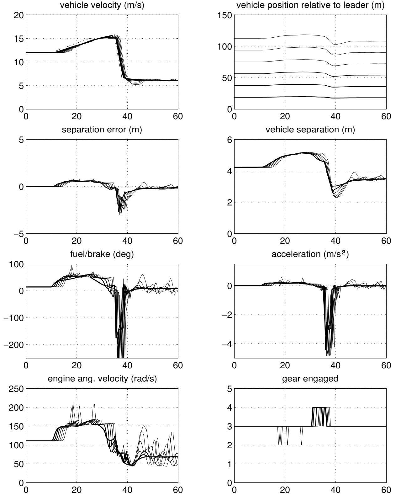
Figure 41: Actuator delay \tau = 0.2 s, backstepping controller with alternative predictor, l = 5 , \Delta = 0.04 s, variable time headway h = 0.1 - 0.2v_r s, and variable separation error gain k = 0.1 + (1 - 0.1)e^{-0.1\delta^2} .
