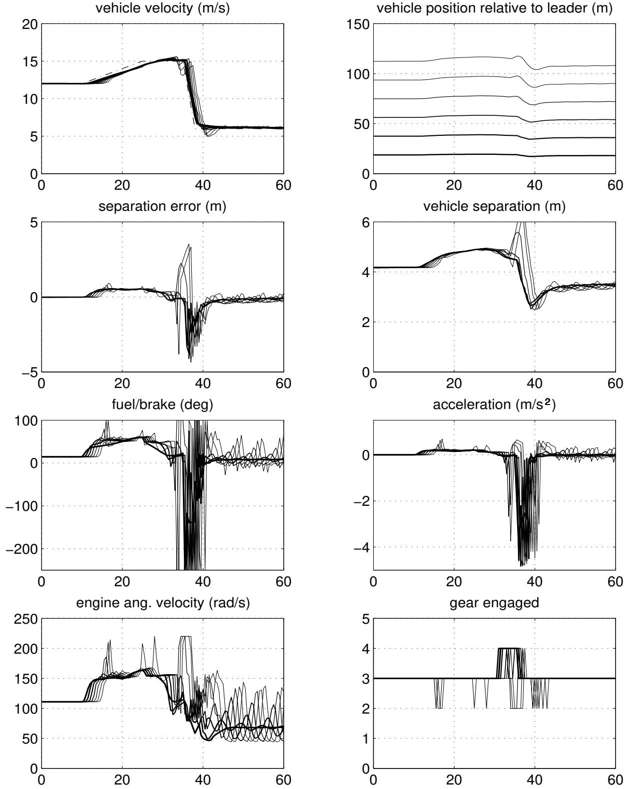
Figure 35: Actuator delay \tau = 0.2 s, backstepping controller with variable time headway h = 0.1 - 0.2v_r s and variable separation error gain k = 0.1 + (1 - 0.1)e^{-0.1\delta^2} .
