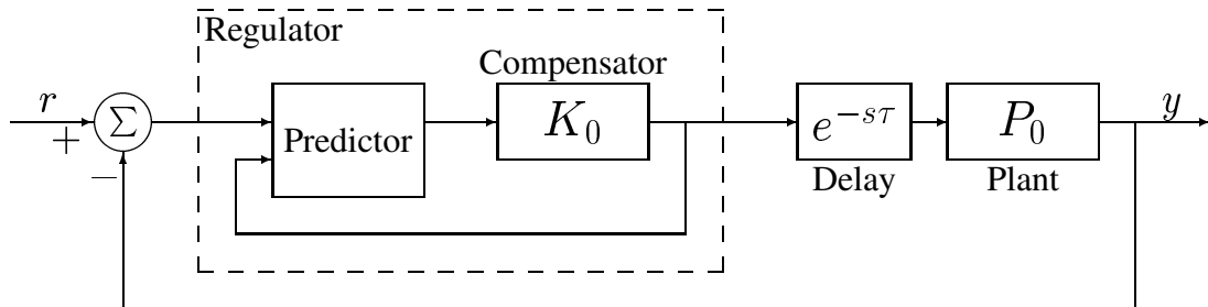
Figure 29: General predictor diagram.
