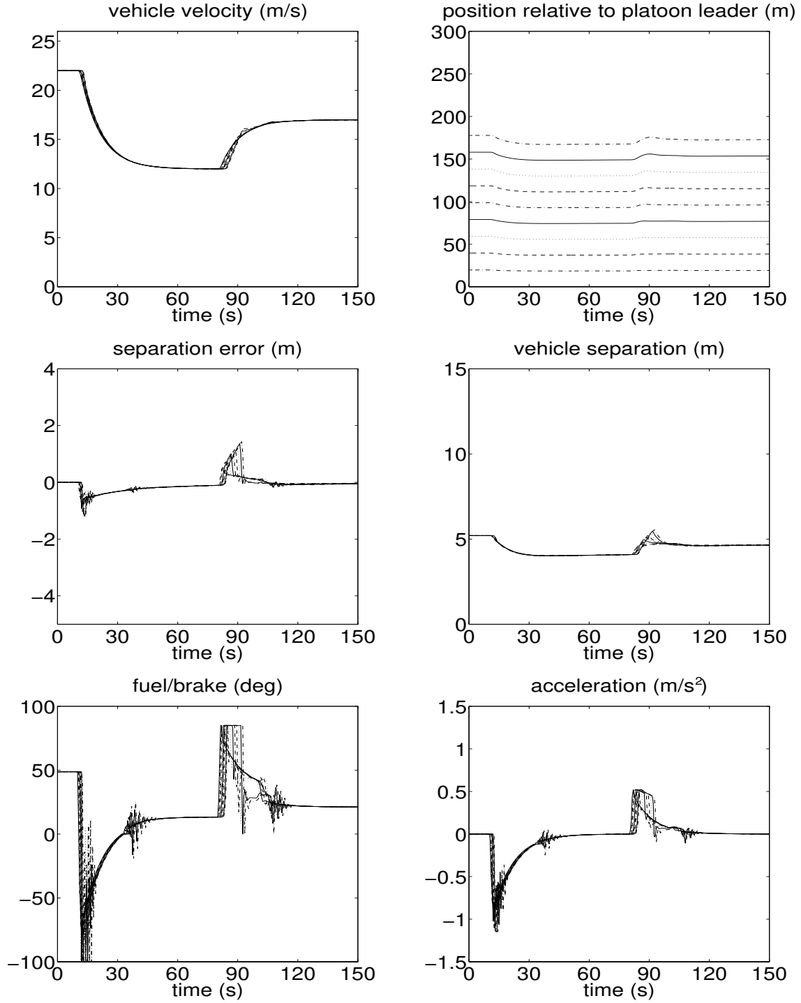
Figure 12: Ten autonomous vehicles, h = \text{sat}(0.1 - 0.2v_r) , variable k , \sigma = 0.1 .
