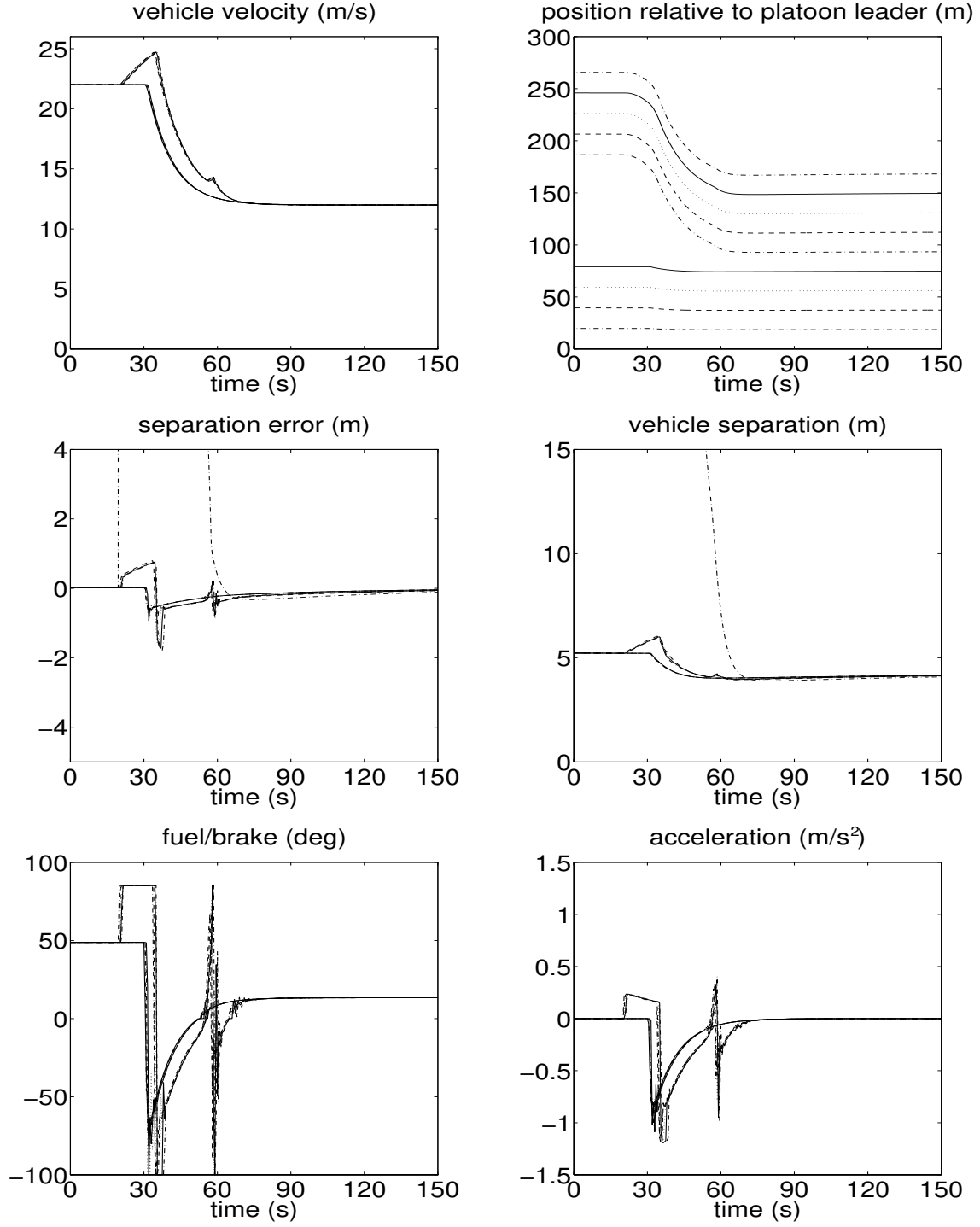
Figure 16: Merge and brake maneuver, h = \text{sat}(0.1 - 0.2v_r) , variable k , \sigma = 0.1 .
