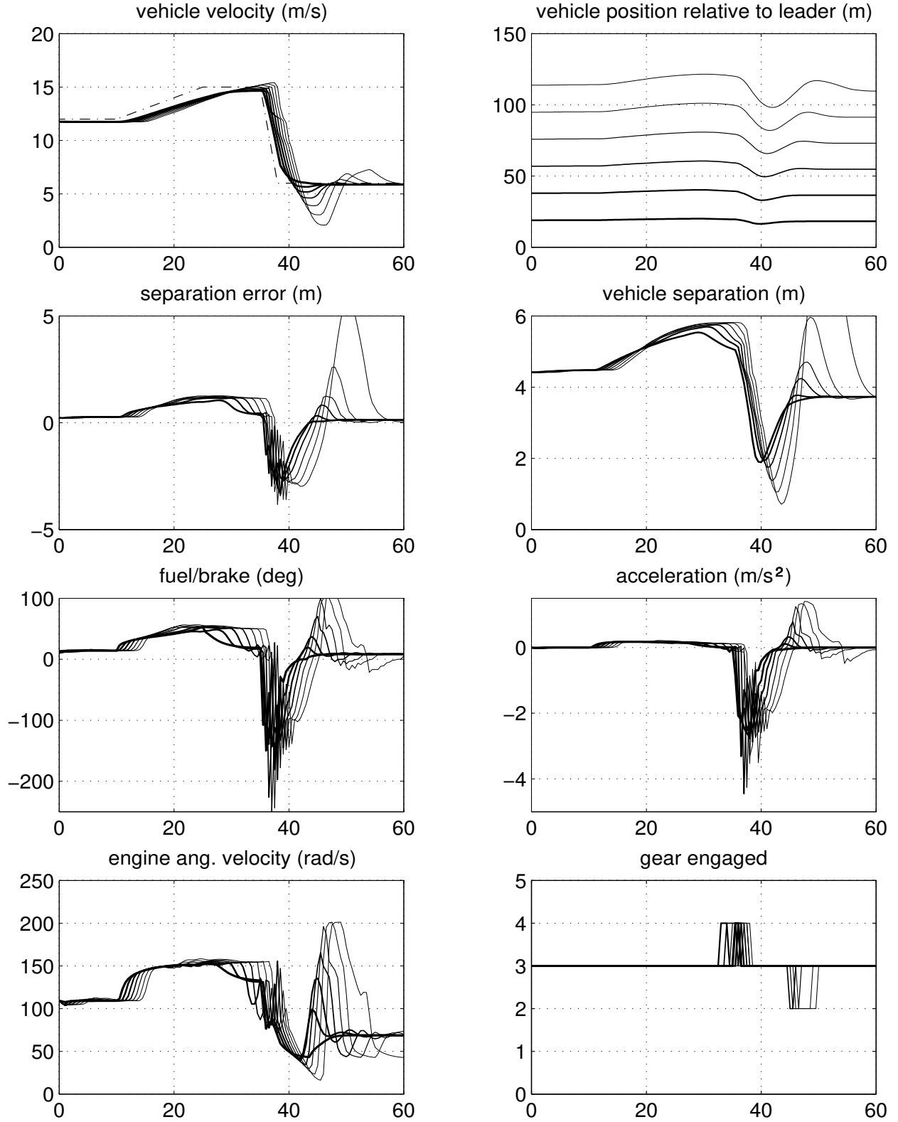
Figure 47: Actuator delay \tau = 0.3 s, PID controller with alternative predictor, l = 5 , \Delta = 0.06 s, variable time headway h = 0.1 - 0.2v_r s, and variable separation error gain k = 0.1 + (1 - 0.1)e^{-0.1\delta^2} .
