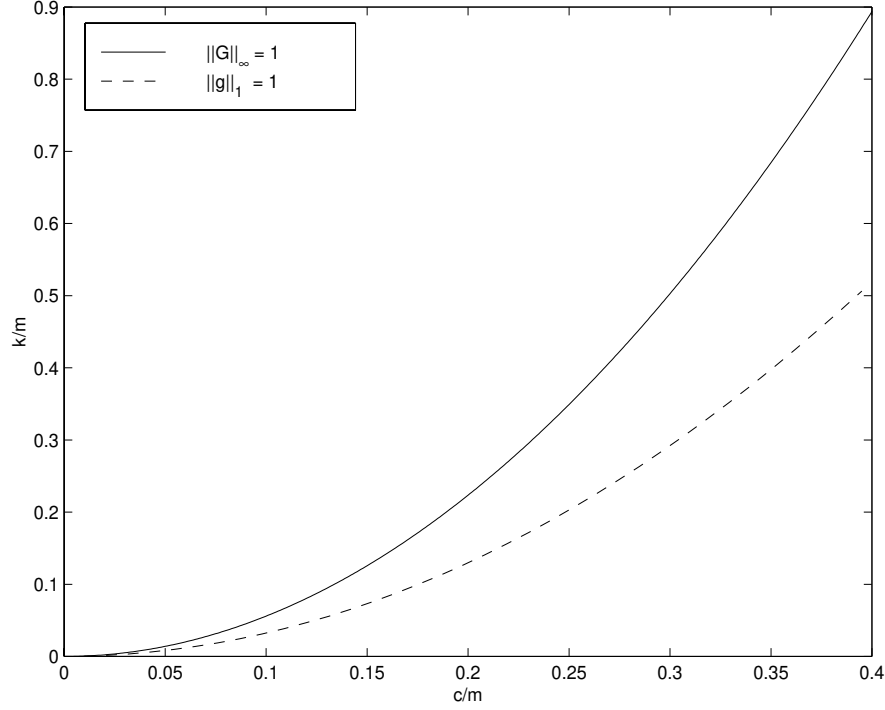
Figure 22: Regions of stability for a 3-vehicle bidirectional platoon with constant spacing.
