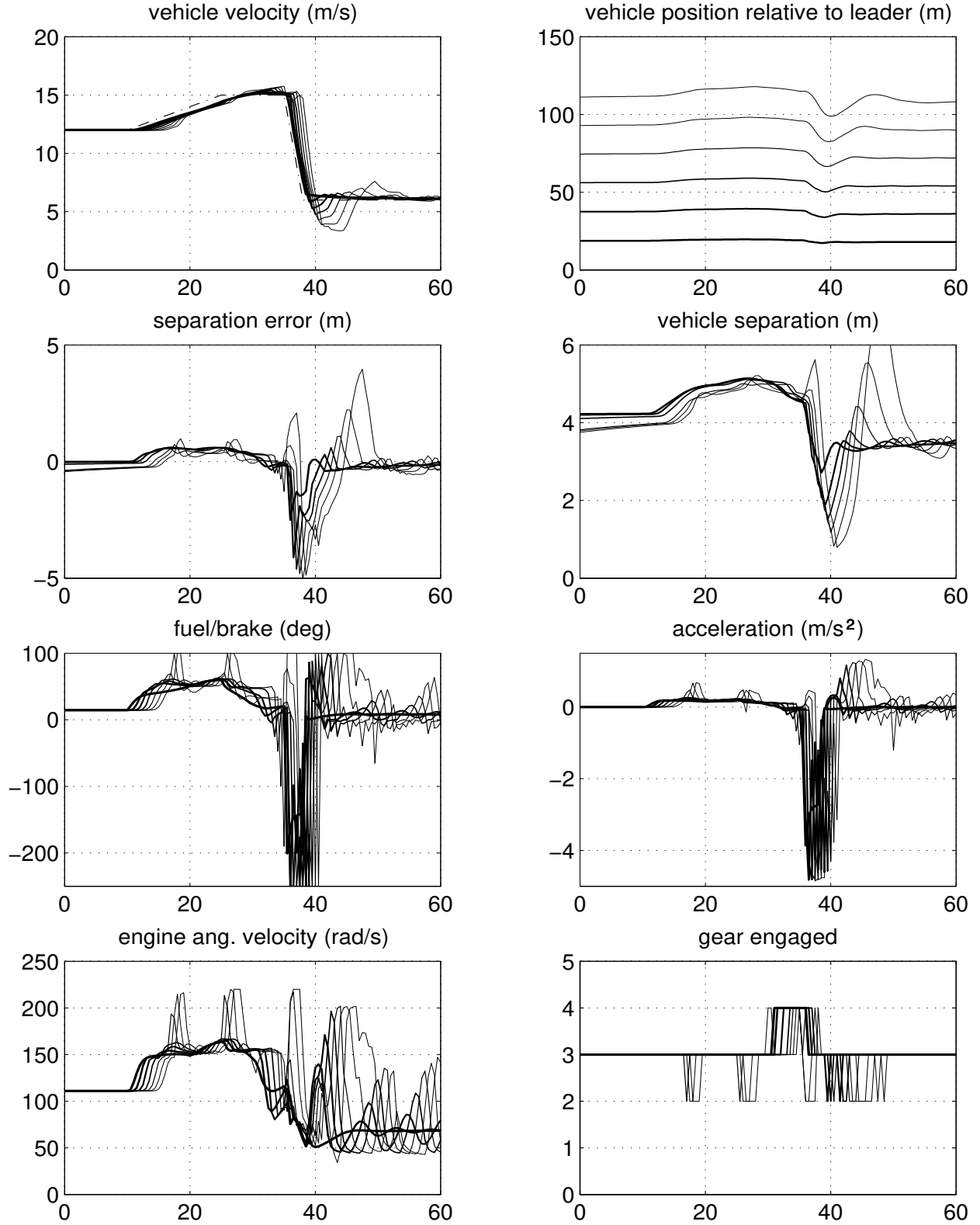
Figure 43: Actuator delay \tau = 0.3 s, backstepping controller with alternative predictor, l = 5 , \Delta = 0.06 s, variable time headway h = 0.1 - 0.2v_r s, and variable separation error gain k = 0.1 + (1 - 0.1)e^{-0.1\delta^2} .
