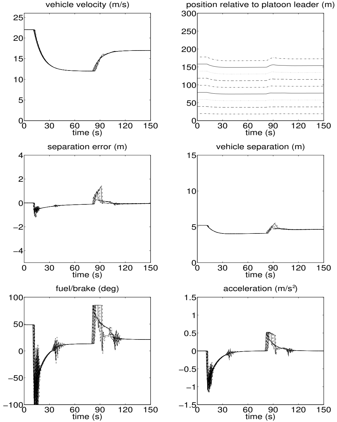
Figure 8: Ten autonomous vehicles, h = \text{sat}(0.1 - 0.2v_r) .
