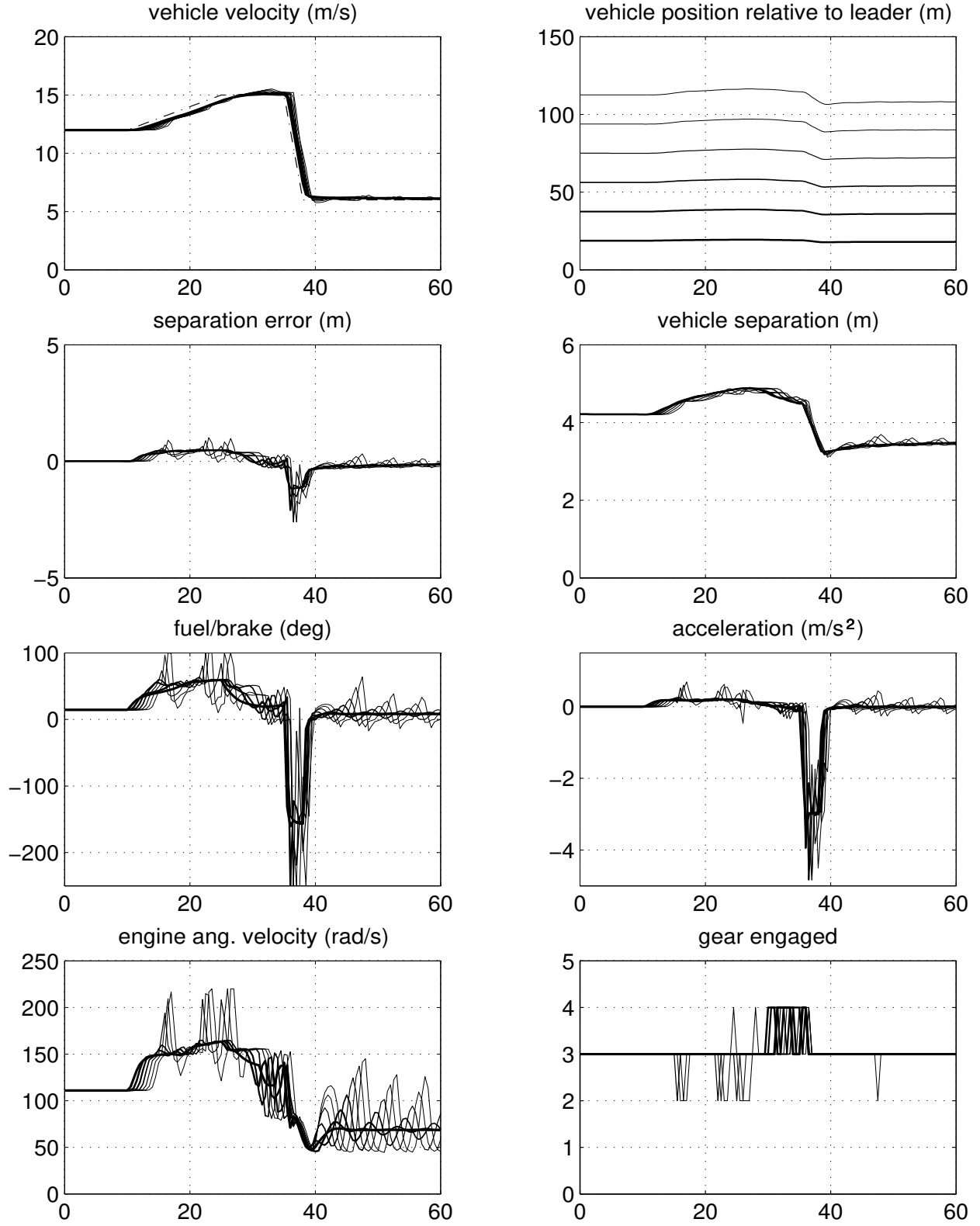
Figure 39: Actuator delay \tau = 0.05 s, original PIQ controller with variable time headway h = 0.1 - 0.2v_r s and variable separation error gain k = 0.1 + (1 - 0.1)e^{-0.1\delta^2} .
