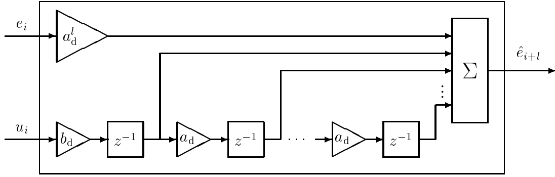
Figure 31: An alternative predictor with true predictive action.
