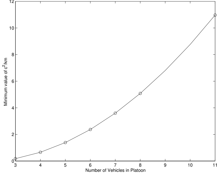
Figure 21: Minimum value of \frac{c^2}{km} required for \|G(jw)\|_\infty \leq 1 .
