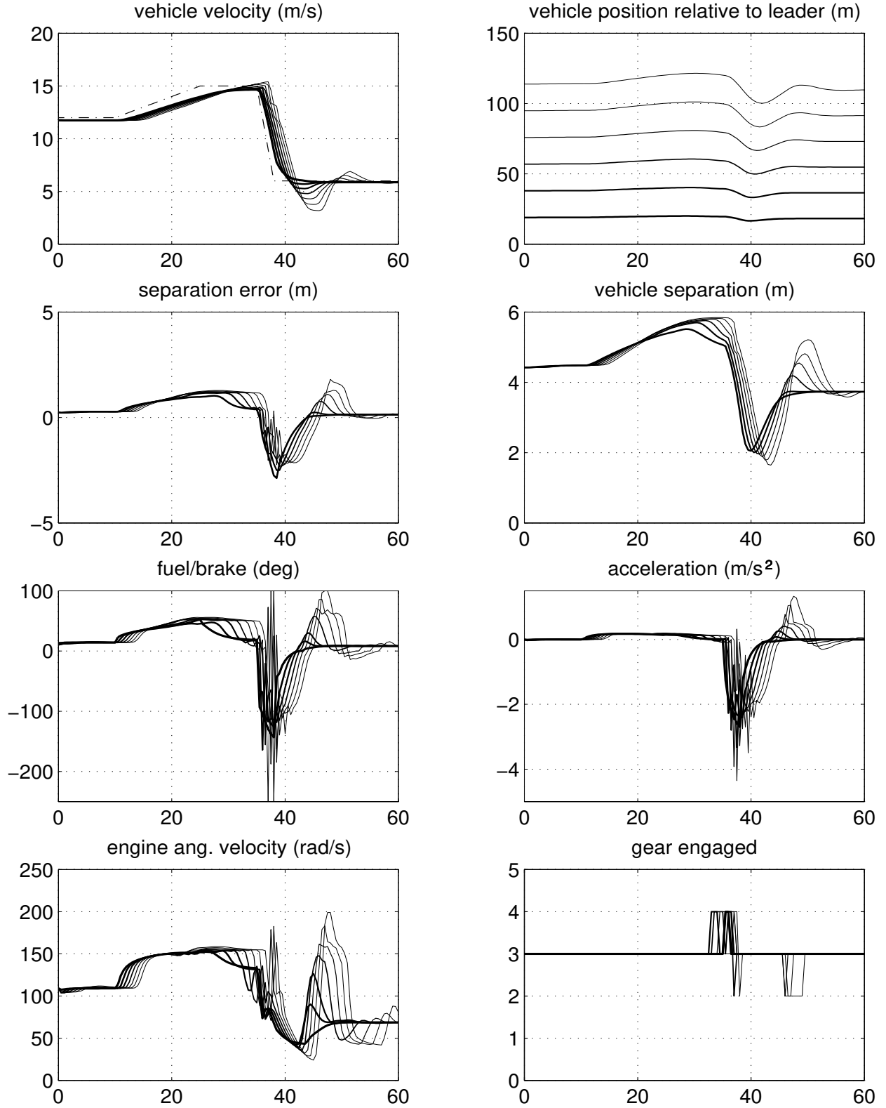
Figure 45: Actuator delay \tau = 0.2 s, PID controller with alternative predictor, l = 5 , \Delta = 0.04 s, variable time headway h = 0.1 - 0.2v_r s, and variable separation error gain k = 0.1 + (1 - 0.1)e^{-0.1\delta^2} .
