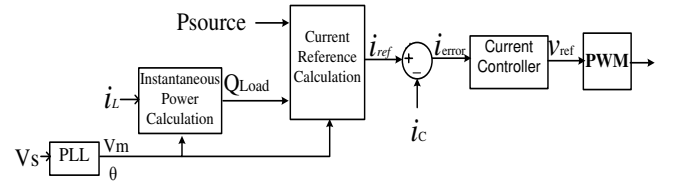
Fig. 11. Control block diagram of the CGCI
