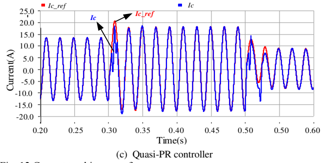
(c) Quasi-PR controller
