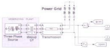
Fig:10 The Power Grid considered for simulation
