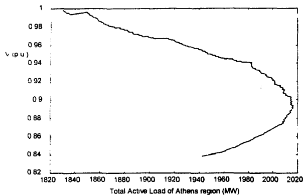
Fig. 3 P-V curve of a 150kV bus in the Athens region (incident of 1996)
