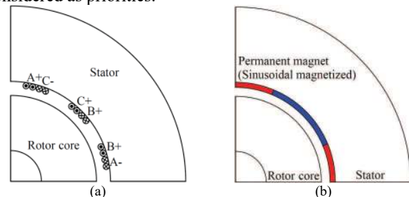
Fig. 8. Simulation of fields without modulation. (a) A model without PMs and stator slots. (b) Simulation of 4th armature reaction magnetic field by PMs.
