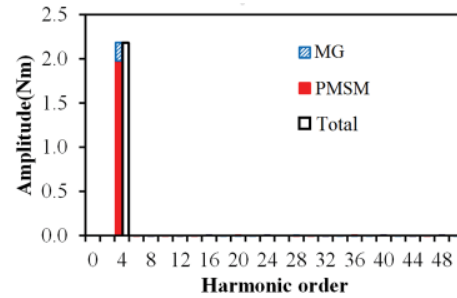
Fig. 11. Torque quantification.
