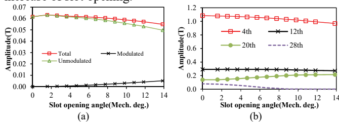
Fig. 12. Influence of slot opening on the field harmonics. (a) Armature reaction harmonics. (b) PM harmonics.
