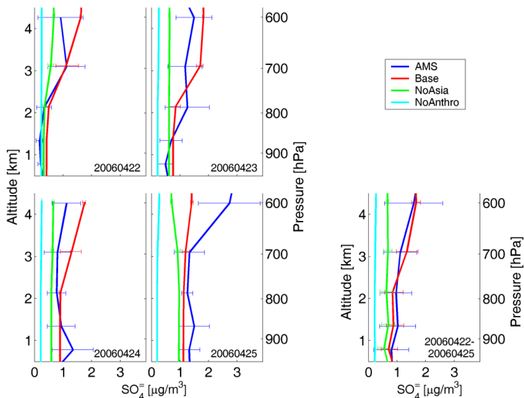
Fig. 9. Cessna Q-AMS \text{SO}_4^- profiles taken 22–25 April 2006. The left-hand panels show individual flight profiles. The right panel shows a mean profile of the same data. Error bars represent one standard deviation of the data. Q-AMS data are at STP and scaled a factor of 1.4 to account for particle size restrictions. A small vertical offset is included between the datasets for visibility.
