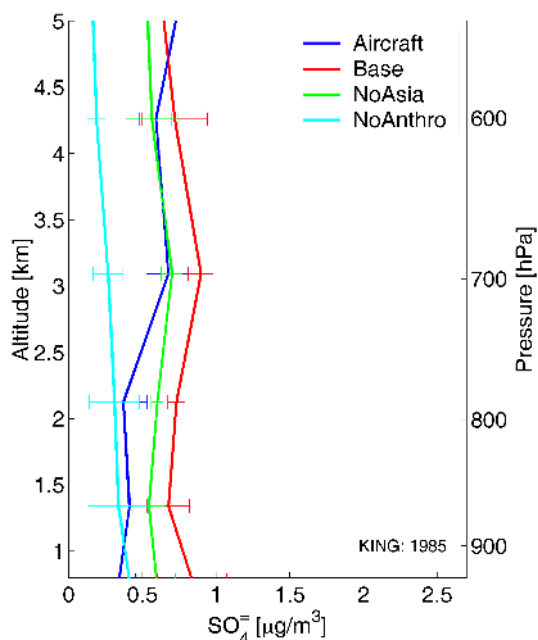
Fig. 7. Average aircraft measurements of \text{SO}_4^- during 1985 King Air flights, within the boundary shown in Fig. 1. Simulated cases of total \text{SO}_4^- include our standard simulation, no East Asian emissions, and no global anthropogenic emissions. All measured and modeled data are at STP. Error bars denote one standard deviation.
