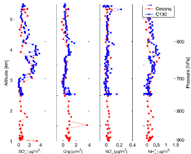
Fig. 3. Aerosol Mass Spectrometer (AMS) measurements from the May 3, 2006 inter-comparison flight over Whistler Peak Station ( 50.1^\circ \text{N} , 122.9^\circ \text{W} ). Cessna data are shown in red. C-130 data are shown in blue. All data at STP. No scaling for the upper size cut of the AMS has been applied to these data.
