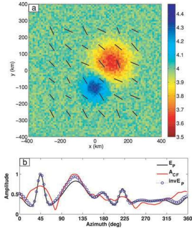
Figure 12. (a) A modified velocity model for the modelling in the inversion using eq. (21). The original velocity model is shown as the case 2 of the model in Fig. 8, which is used for the calculation of the cross-correlation functions from eq. (1). The amplitude of the velocity anomaly (isotropic part) in the modified model is 75 per cent of that in the original velocity model. And a maximum of 0.05 \text{ km s}^{-1} random noise is added to the isotropic part of the modified velocity model. For the azimuthal anisotropic part, we add a maximum of 25^\circ random noise to the azimuth of the fast propagation direction and a maximum of 2 per cent random noise to the amplitude of azimuthal anisotropy (originally 5 per cent). (b) Recovery of the ambient noise energy (blue open circles) when using the modified velocity model (a) in the inversion but the original velocity model for calculating the cross-correlation functions. In (b), the input ambient noise energy is shown as the black curve and the red curve shows the amplitude of the cross-correlation functions.
