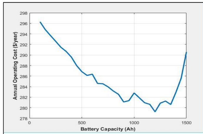
Figure 4. Optimum battery capacity with minimum operating cost
