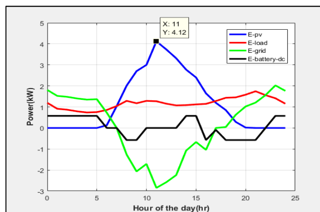
Figure 3. Energy transfer sequences of PV system
