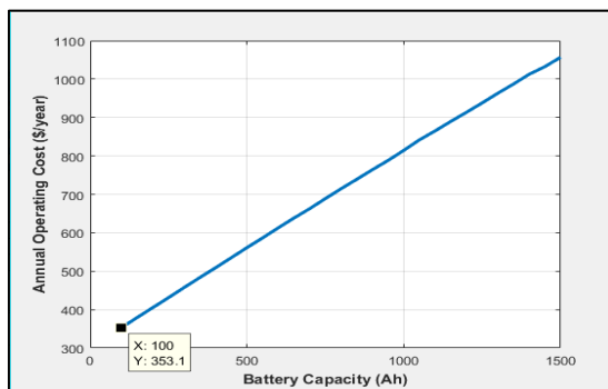
Figure 6. Optimum battery capacity with minimum operating cost
