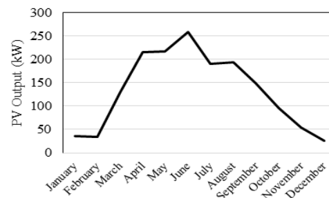
Figure 1. Average monthly PV output profile
