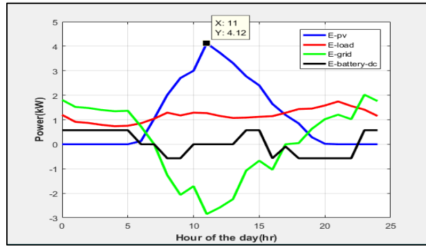
Figure 5. Energy transfer sequence of PV system
