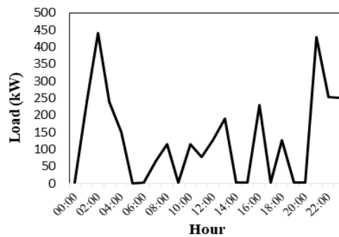
Figure 2. Average hourly load consumption data
