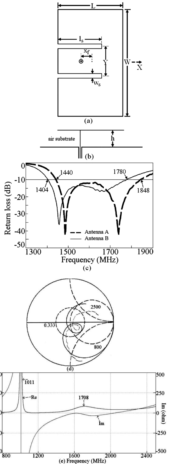
Fig. 1 (a) Top and (b) side views of E-shaped MSA, its (c) return loss plots [6], (d) input impedance, (—) simulated, (---) measured and (e) simulated resonance curve plots for optimized E-shaped MSA
