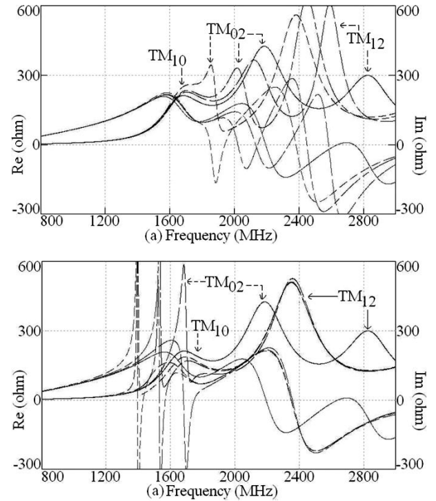
Fig. 3 Resonance curve plots for (a) ( \text{—} ) l_s = 0 , ( \text{---} ) l_s = 1.5 , ( \text{- - -} ) l_s = 2.0 , ( \text{- - -} ) l_s = 2.5 , (b) ( \text{—} ) l_s = 0 , ( \text{---} ) l_s = 3.0 , ( \text{- - -} ) l_s = 3.5 , ( \text{- - -} ) l_s = 4.0 , for E-shaped MSA
