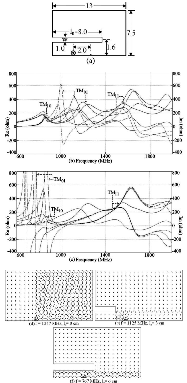
Fig. 7 (a) Rectangular slot cut RMSA, its resonance curve plots for (b) (—) l_s = 0 , (---) l_s = 2 , (---) l_s = 3 , (---) l_s = 4 , (c) (—) l_s = 0 , (---) l_s = 5 , (---) l_s = 6 , (---) l_s = 7 , and (d – f) surface current distribution at TM_{01} mode for different slot length
