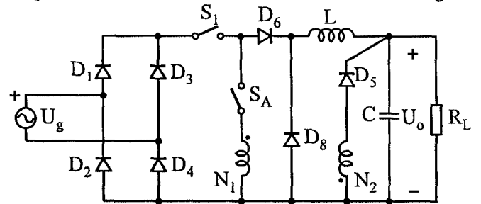
Fig. 6 - Proposed integrated buck-flyback converter
