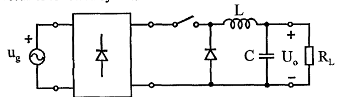
Fig. 1 - Buck-type preregulator
