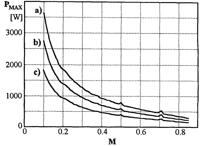
Fig. 5 - Maximum input power as a function of voltage conversion ratio M in case of sinusoidal-current reference modulation.
