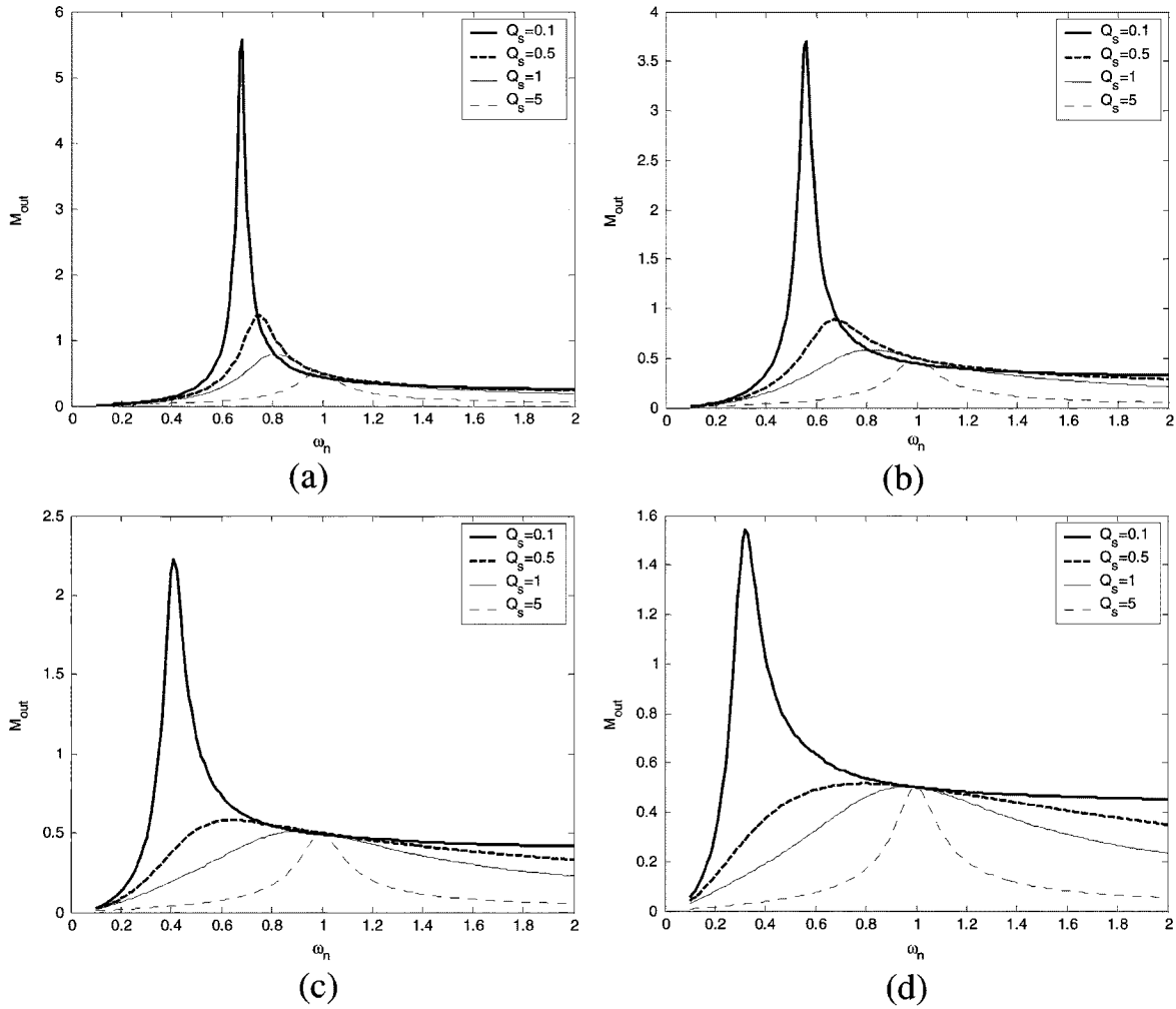
Fig. 6. M_{out} as a function of \omega_n for various Q_s values. (a) A = 1 , (b) A = 2 , (c) A = 5 , and (d) A = 10 .
