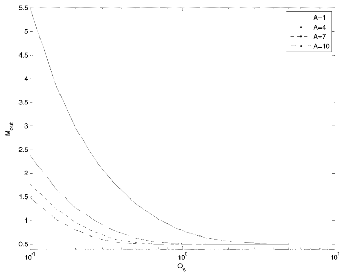
Fig. 8. Converter gain as a function of series Q -factor for numerous inductor ratios.
