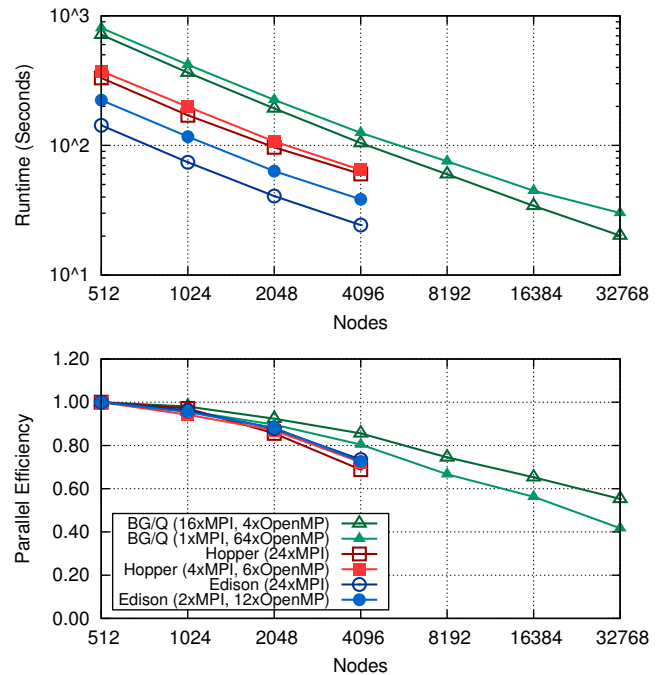
Figure 7: FLASH Performance
