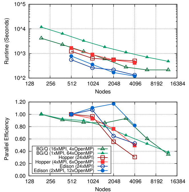
Figure 5: MILC Performance
