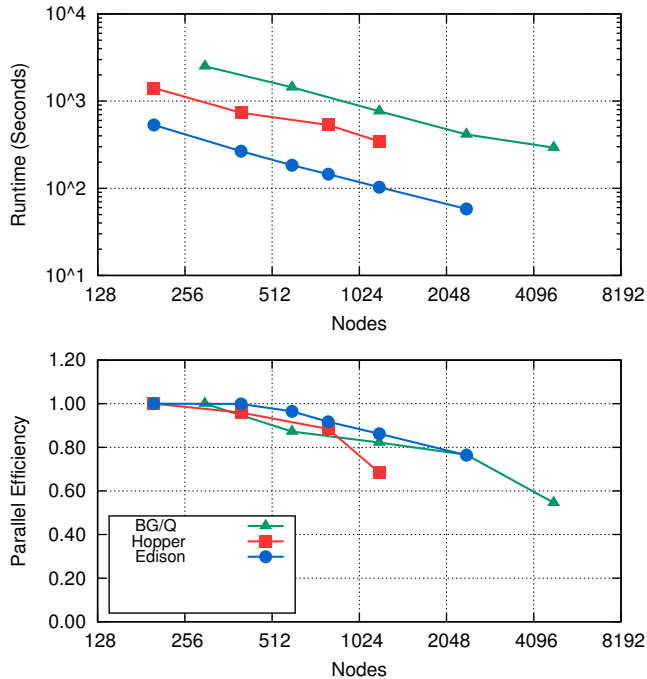
Figure 6: GTC Performance
