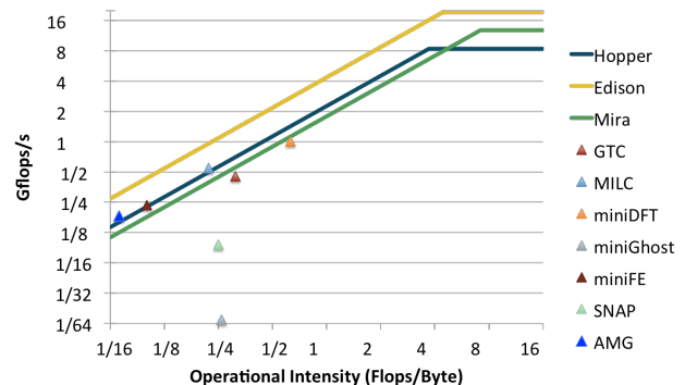
Figure 3: Roofline model of test systems with NERSC8/Trinity benchmarks. For each of the test systems, the plot shows a roofline model (colored lines) constructed from the peak floating point performance per core of each system and the measured memory bandwidth from the STREAM benchmark. Each colored triangular symbol marks the results obtained from Hopper for test cases that run on order 1000 nodes.
