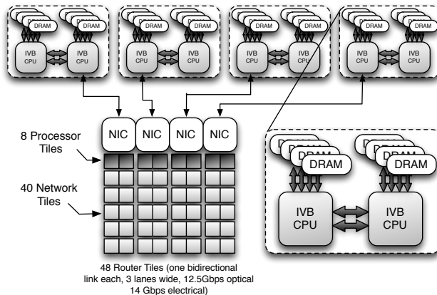
Figure 2: Cray XC30 Node Architecture
