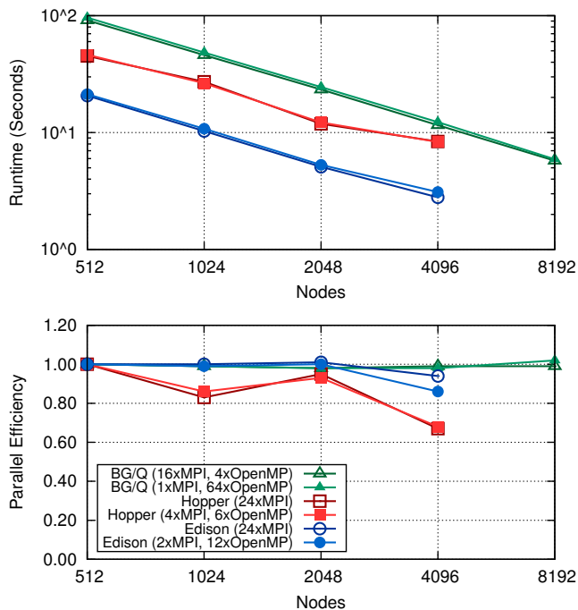
Figure 8: MiniFE Performance
