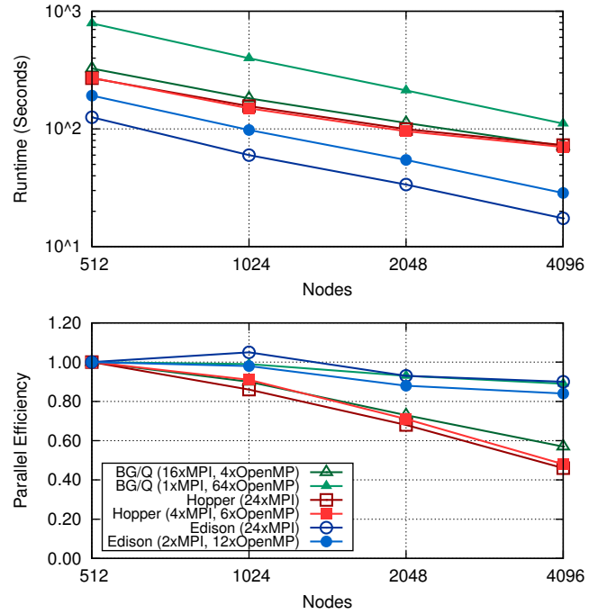
Figure 9: UMT Performance
