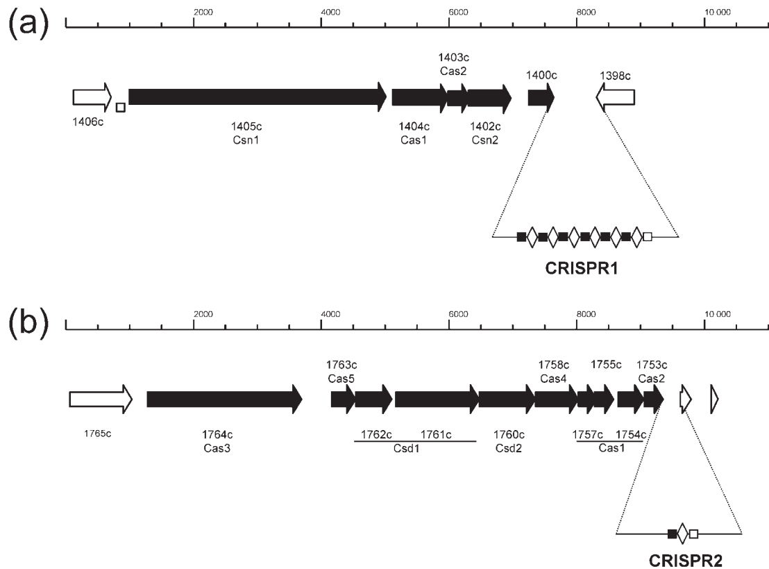
Fig. 1. Organization of CRISPR1 (a) and CRISPR2 (b) arrays and associated genes in S. mutans UA159. Lines below the ORF numbers show the size that the gene would have if the frame shift or stop codons (see text) were removed. CRISPR repeats are indicated by boxes (black, conserved; white, degenerated). Spacers are indicated by diamonds.
