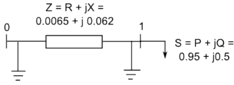
Fig. 2. A two-node system with fixed real and reactive demand at bus 1.
