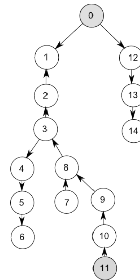
Fig. 4. The 15-bus example of section IV. Grey nodes indicate locations of flexible resources. The arrows indicate the direction of flow of real power for the optimal solution for both the case with and without line capacity limits.
