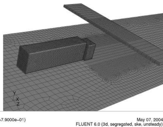
Fig. 8. 3D test surface mesh
