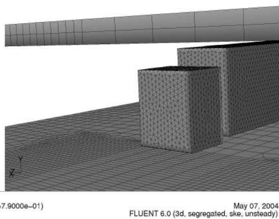
Fig. 9. 3D test surface mesh
