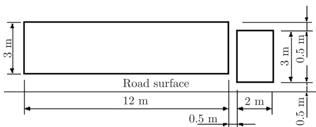
Fig. 4. Lorry geometry
